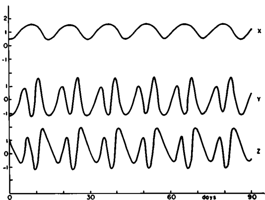
Fig. 3. Same as Fig. 2; stable periodic solution with G = 0.8 . Normal scale for X .
