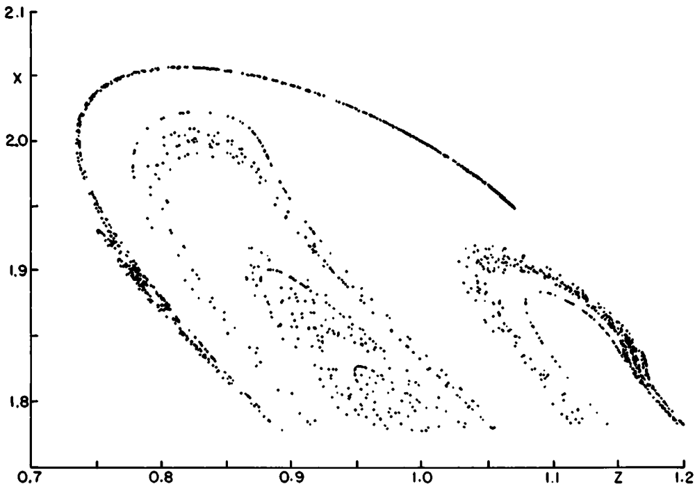
Fig. 8. Portion of intersection shown in Fig. 7, enlarged 10 times, as indicated by 2000 intersection points.
