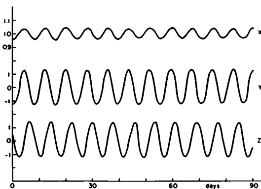
Fig. 2. Variations of X , Y , Z during 90 day interval, in solution of eqs. (1)–(3) with a = 0.25 , b = 4.0 , and F = 8.0 ; stable periodic solution with G = 0.2 . Note expanded scale for X , relative to Y and Z .
