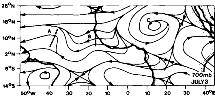
Fig. 8. Streamline map at 700 mb for 12Z July 3, 1974.
