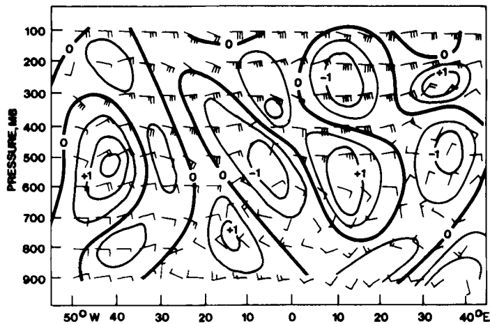
Fig. 11. Vertical cross section along 14°N latitude for 12Z July 5, 1974. Isoleths represent isotherms of temperature deviations in °C; contour intervals are 0.5 °C. Wind barbs are total horizontal wind components; full barb is equal to 5 ms -1 .
