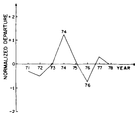
Fig. 3. Normalized departure of annual precipitation based on 58 stations in north east Brazil.
