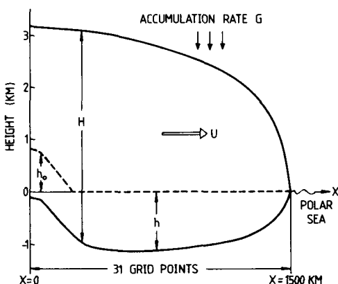
Fig. 1. Geometry of the model ice sheet.
