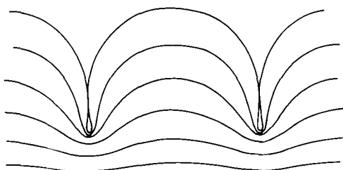
Fig. 3. Streamlines of capillary waves of finite amplitude—from Crapper (1957). Each of the lower streamlines can be taken as the surface of a capillary wave of lesser steepness (by permission of Cambridge University Press).
