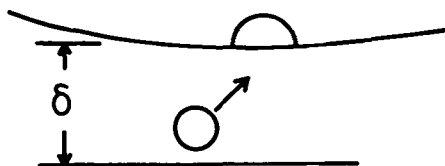
Fig. 1. Sketch of a fluid particle moving through the viscous sublayer and finally deforming the interface.
