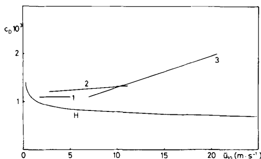
Fig. 2. Roughness of the sea surface. Comparison between measured drag coefficients c_D = u_*^2/\bar{u}_{10m}^2 (numbered lines) and hydrodynamical smooth flow (curve marked H ). The implication is that the increase of momentum flow compared to smooth flow is brought about by "form" drag of gravity waves and ripples. The average value at moderate wind speeds is fairly well known both from direct and profile measurements, while the value at high wind speeds is based on few direct measurements. Results are taken from (1) Dittmer (1977), (2) Brooks and Krügermeyer (1972), (3) Smith and Banke (1975).
