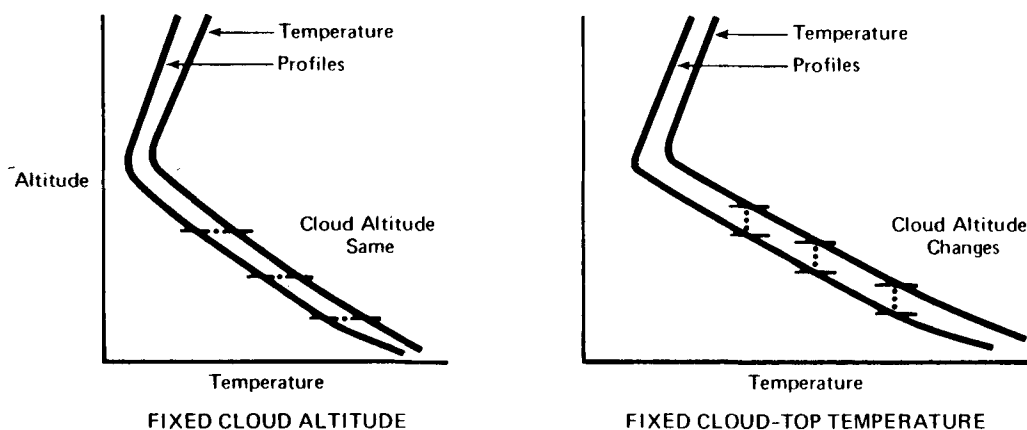
Fig. 1. Comparison of cloud altitude for the fixed cloud altitude model and the fixed cloud-top temperature model.
