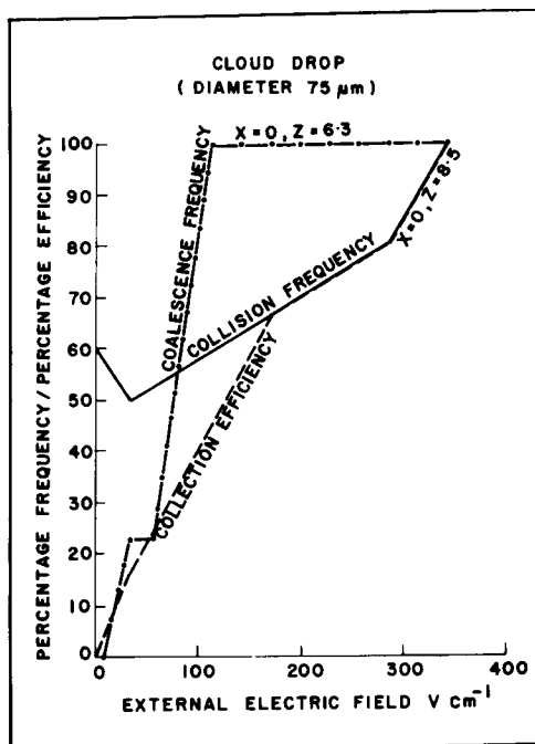
Fig. 5. Collision frequency, coalescence frequency and collection efficiency of equal size drops in mustard oil.
