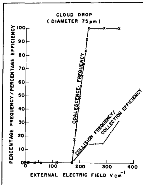
Fig. 7. Same as Fig. 5. for unequal size drops.
