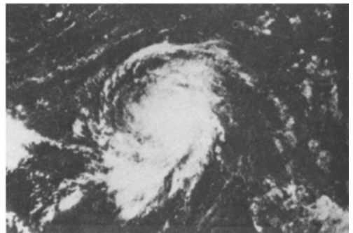
NASA ATS 111 16 AUG 69 1930Z 40B
