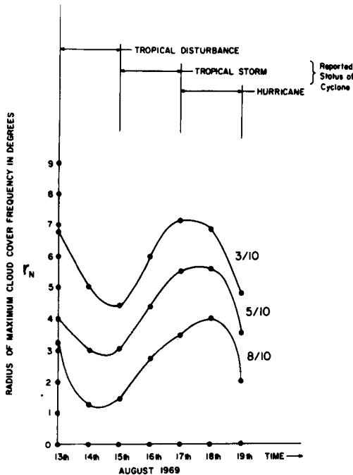
Fig. 4a. Variation of r_N with time for N equals three-, five- and eight-tenths satellite-observed cloud cover for hurricane Debbie. The information here is from Fig. 3.
