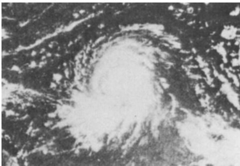
NASA ATS 111 16 AUG 69 1454Z 26B
