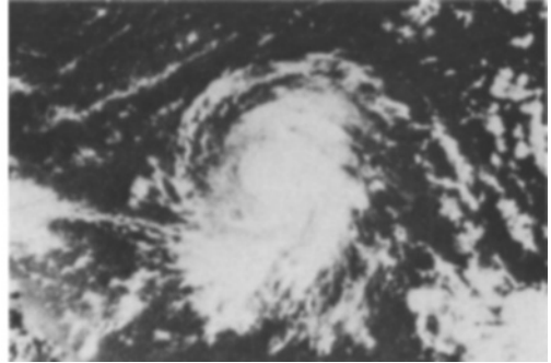
NASA ATS 111 16 AUG 69 1741Z 39B
