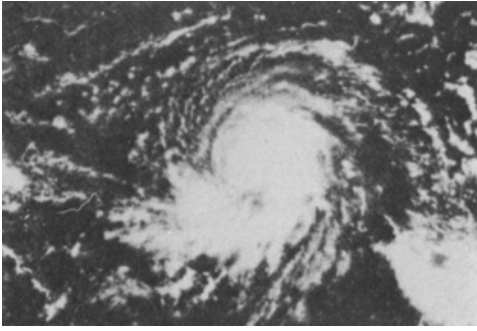
NASA ATS 111 16 AUG 69 1233Z 15B
