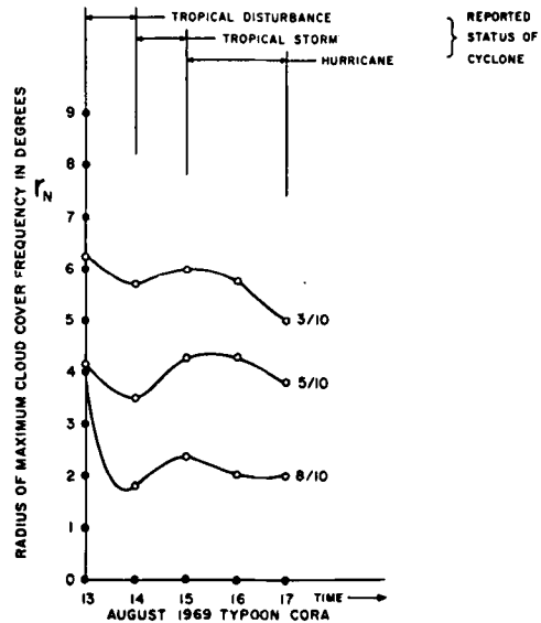
Fig. 4b. Variation of r_N with time for N equals three-, five- and eight-tenths satellite-observed cloud cover for typhoon Cora, August 1969.
