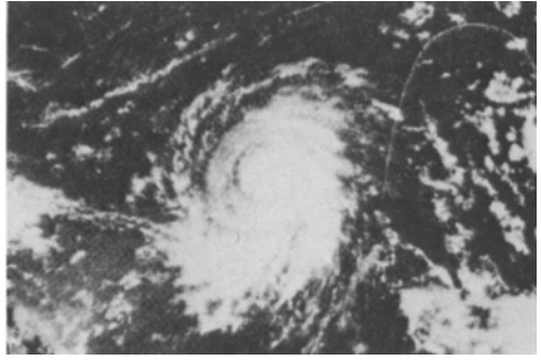
NASA ATS 111 16 AUG 69 1650Z 35B
