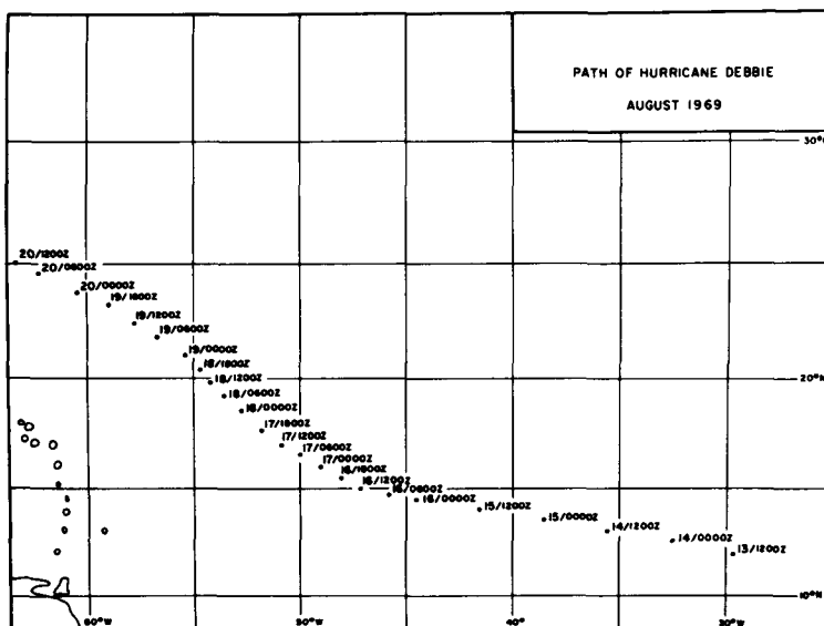
Fig. 1. Path of hurricane Debbie; August 13–August 20, 1969.
