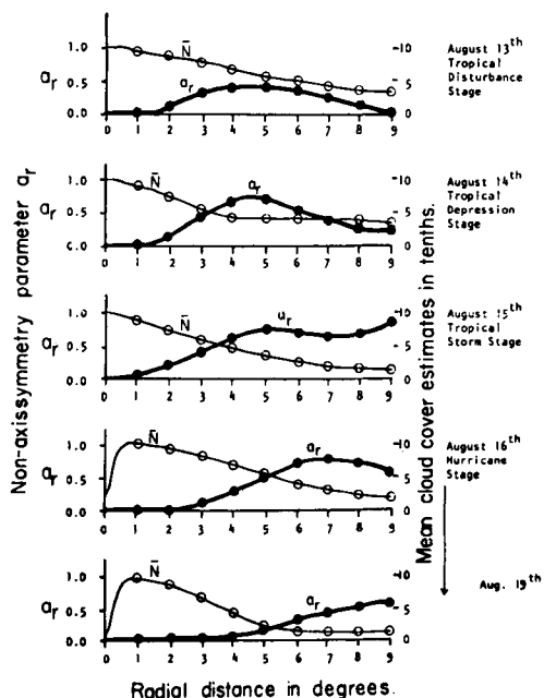
Fig. 7. Graphs of a_r as a function radial distance and time. Graphs of \bar{N} are also indicated on the graphs.
