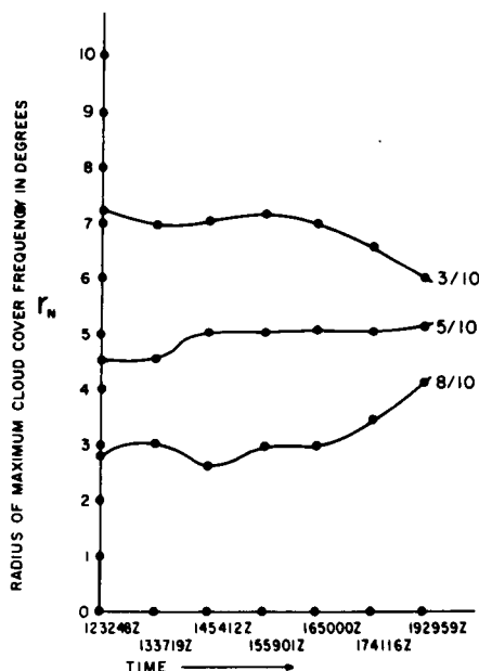
Fig. 9. Graphs of three-, five- and eight-tenths cloud cover as function of radial distances and time computed from a frequency distribution of cloud cover amounts for the hourly data.
