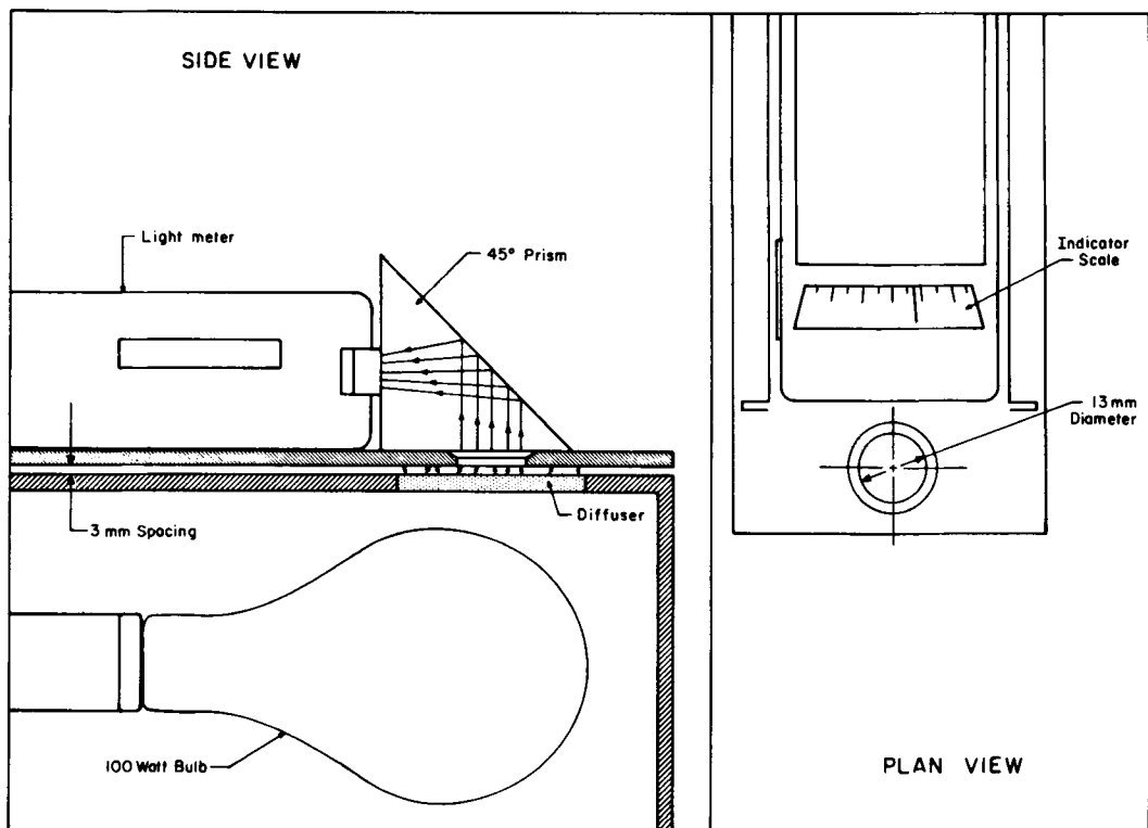
Fig. 2. Photometer arrangement.
