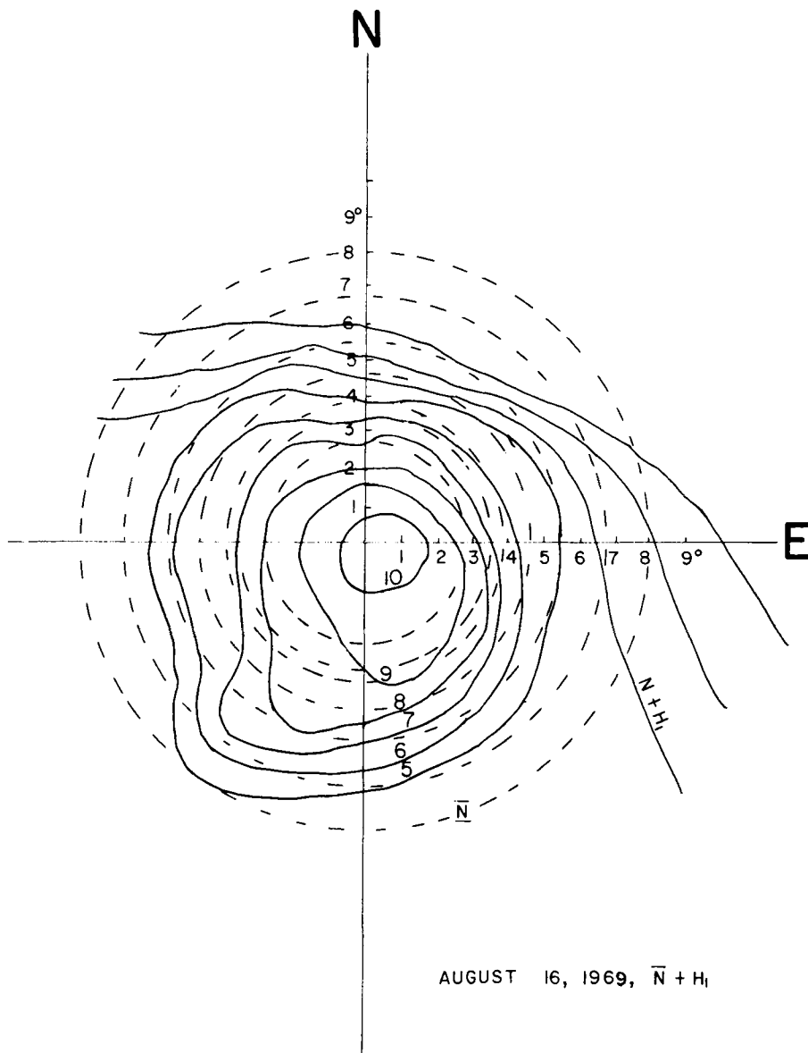
Fig. 9b. Cloud distribution obtained by the addition of the mean cloud amount N and the amplitude of the first harmonic.
