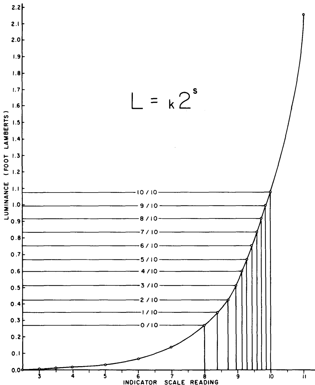
Fig. 4. Calibration curve for the determination of satellite observed cloud cover.
