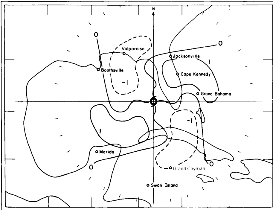
Fig. 11b. Polar diagram showing the distribution of amplitude and phase angles for the second harmonic component for hurricane Abby.
