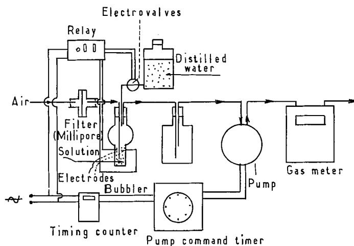
Fig. 3. Schema of SO 2 sampling device.
