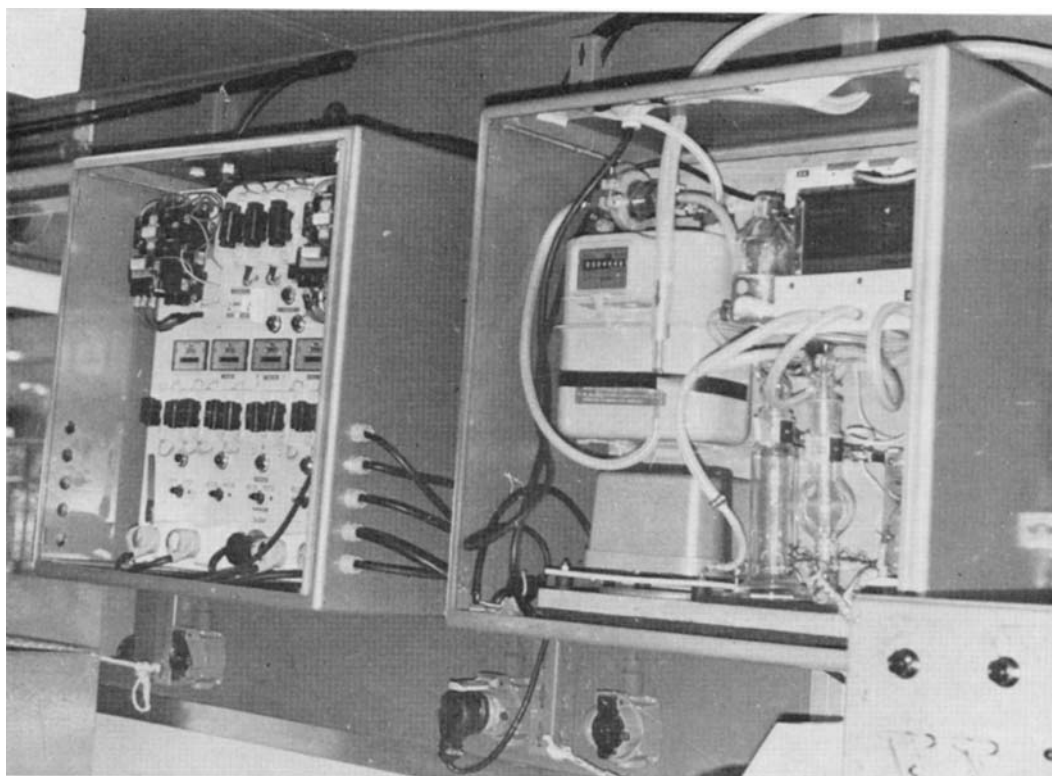
Fig. 2. Electrical control (on the left) and \text{SO}_2 sampling device (on the right).
