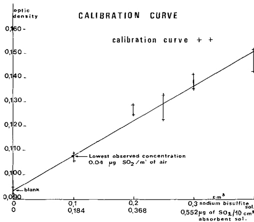
Fig. 4. Calibration curve.
