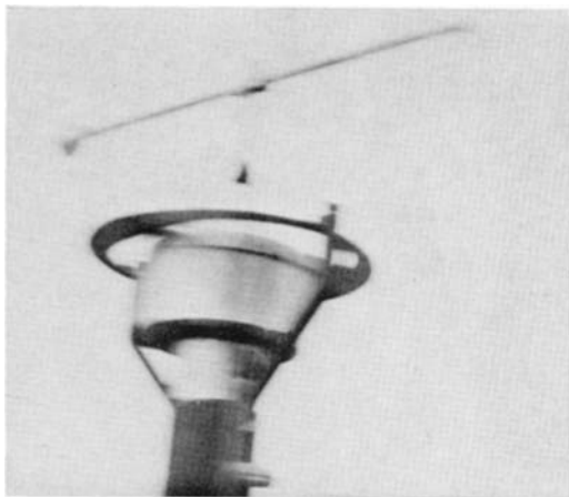
Fig. 1. System to avoid \text{SO}_2 sampling from contaminations by ship exhausts.
