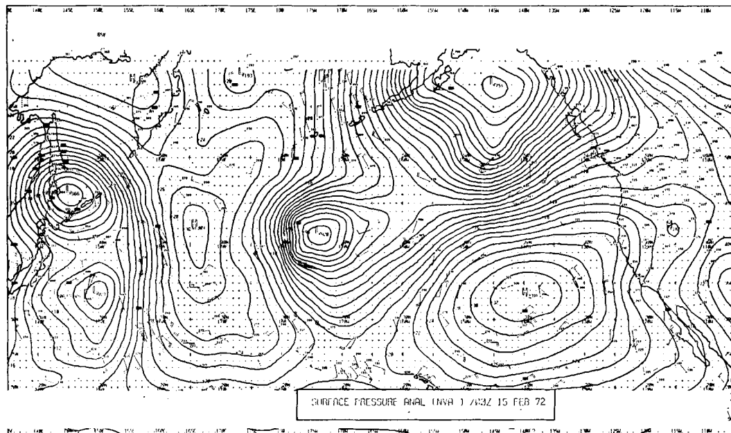
Fig. 2. Sea level pressure at OOO on 15 February 1972. This analysis is the result of a two-dimensional NVA adjustment that has incorporated both wind and pressure reports. The observed winds (knots) and pressure (tenths of a millibar) rejected during analysis have been denoted by dotted bars and blocked numbers, respectively.
