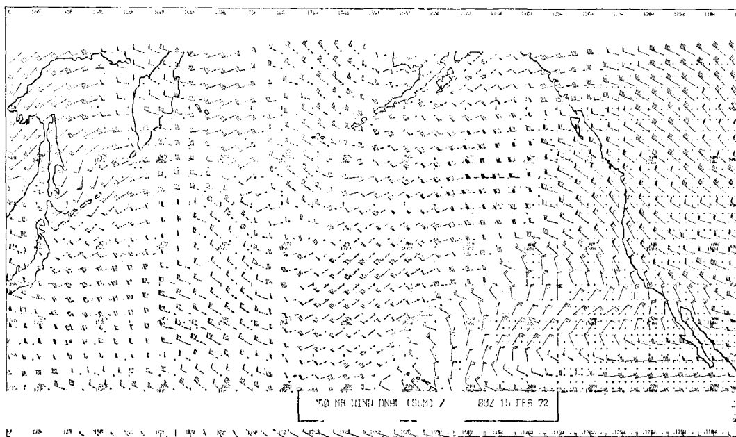
Fig. 4. 250 mb winds (knots) which serve as the upper boundary condition for construction of the intermediate levels. This analysis is derived by the SCM scheme and has not been subjected to variational adjustment.
