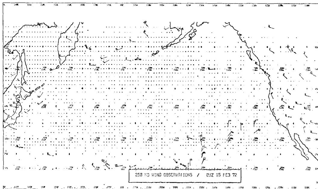
Fig. 5. The wind observations (knots) used by the SCM scheme to construct the 250 mb analysis. The guess field for the SCM above 20 N is the 12 hour forecast from the primitive equation model.
