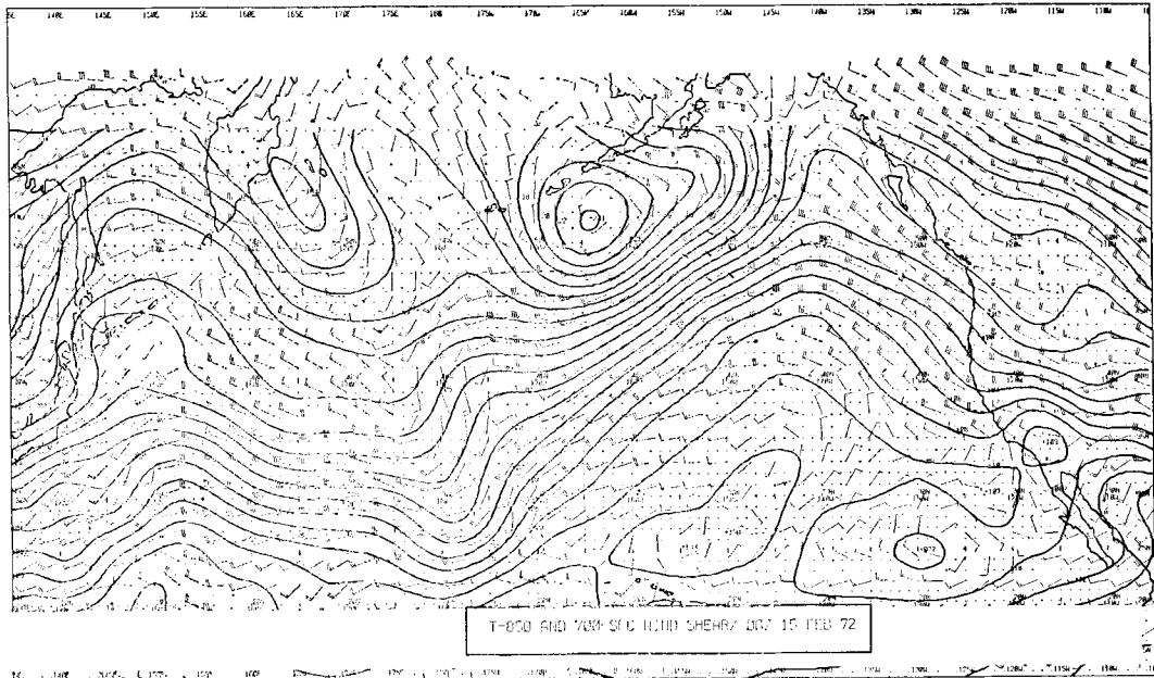
Fig. 12. Same as Fig. 11 except weights used in accord with eq. (23).
