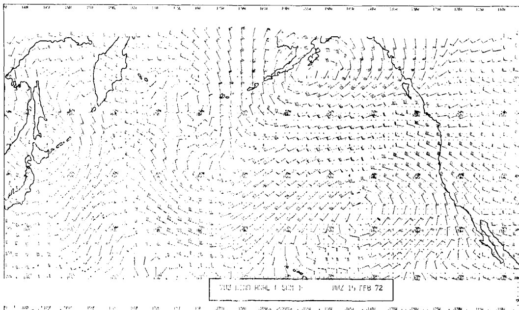
Fig. 8. 700 mb wind analysis (knots) by SCM scheme, \bar{V} (700 mb).
