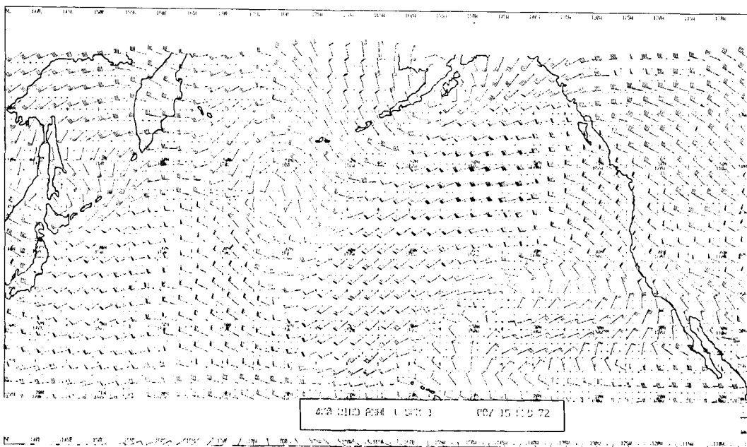
Fig. 9. 400 mb wind analysis (knots) by SCM scheme \bar{V} (400 mb).
