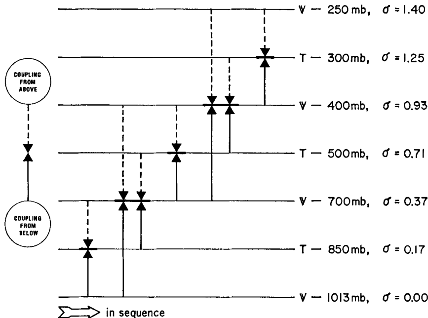
Fig. 1. Schematic representation of "Ascent-Cascade" process of upper-air analysis. The fields at the surface and 250 mb are control or anchor levels. Analysis begins at 850 mb and proceeds to 300 mb (sequencing from bottom to top and left to right in the figure). After completion of a cycle from 850 to 300 mb, the procedure is repeated using the adjusted values as input.
