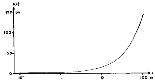
Fig. 1. Inversion height h(x) versus fetch x .
