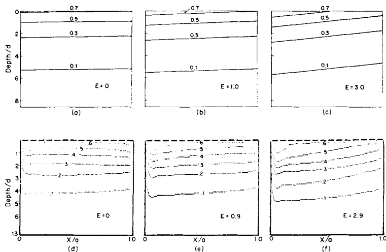
Fig. 3. East/west temperature sections at 32^\circ N from the analytical model (a - c) compared with the numerical results (d - f) of Bryan & Cox (1967). From left to right E=0 corresponds to no wind, E=1 to moderate wind, and E=3 to strong wind. The parameters K=1 and C=0.2 are held fixed.
