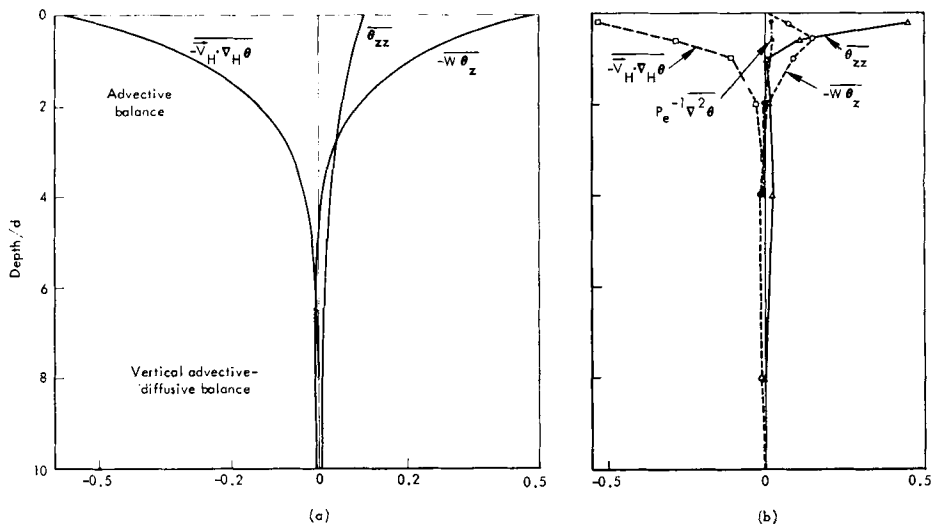
Fig. 6. East/west average of heat balance components at 33^\circ \text{N} for K = E = 1 , C = 0.2 ; (a) analytical model, (b) Bryan & Cox (1968). The surface z = 0 in the analytical model corresponds roughly to the point where -w\theta_z is a maximum in the numerical model.
