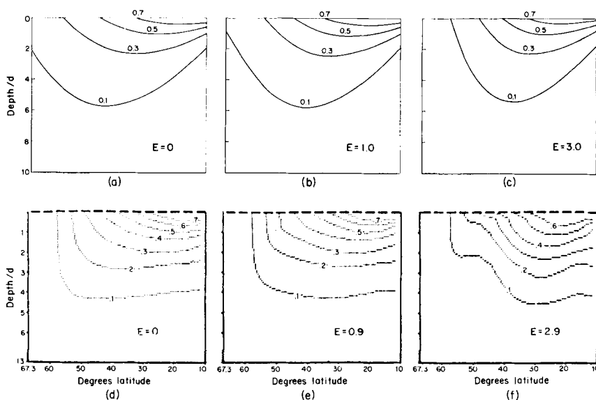
Fig. 4. North/south temperature sections bisecting the basin, (a - c) analytical model, (d - f) Bryan & Cox (1967). From left to right E=0 corresponds to no wind, E=1 to moderate wind, and E=3 to strong wind. The parameters K=1 and C=0.2 are held fixed.
