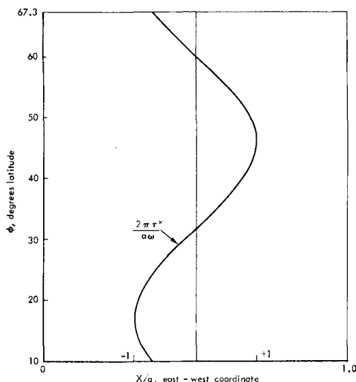
Fig. 1. Model basin and x -component \tau^x of the applied wind stress.
