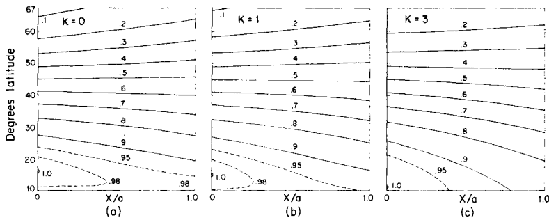
Fig. 5. Horizontal temperatures patterns at z = 0 . From left to right, K = 0 corresponds to no diffusion, K = 1 to moderate diffusion, and K = 3 to strong diffusion. The parameters E = 1 and C = 0.2 are held fixed. Note the lack of appreciable difference among the distributions.
