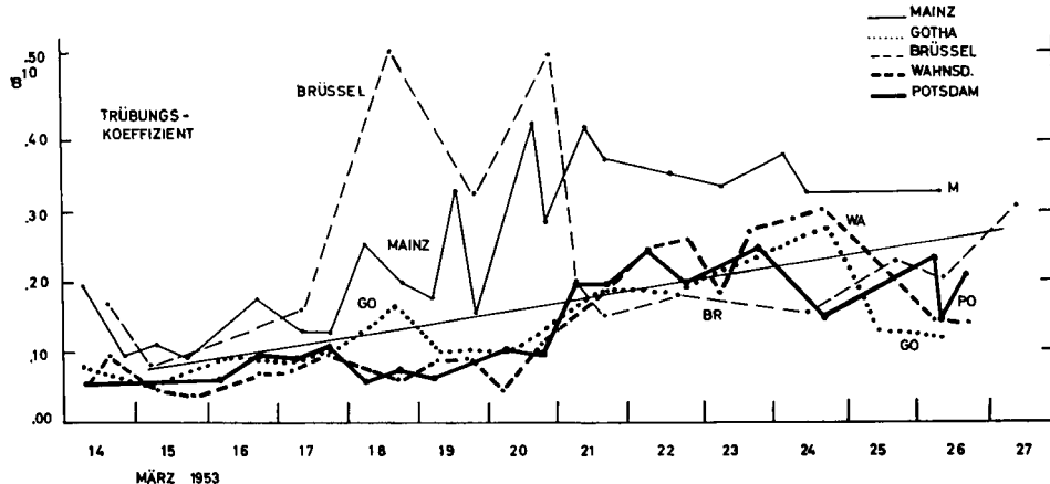
Fig. 6. Turbidity increase in central Europe, probably due to manmade pollution, in a period of weak circulation.
