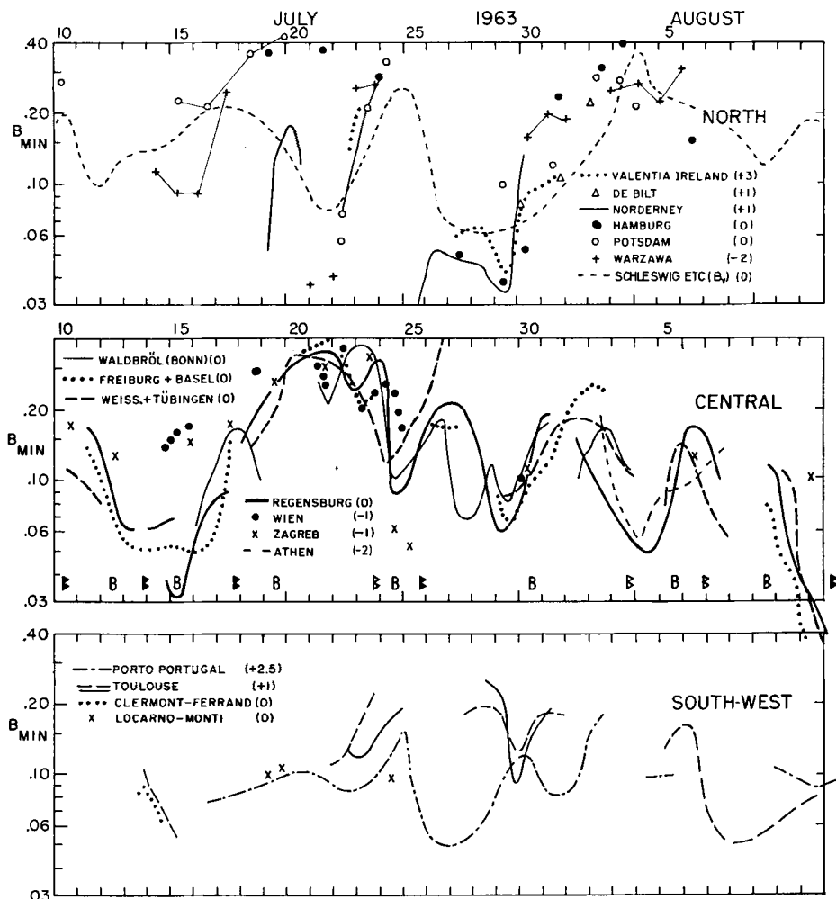
Fig. 4. Turbidity in the northern, central, and southwestern part of Central Europe, July 10 to August 12, 1963. Dashed curve in upper part, logarithmic averaged values of B_V (assuming H_D = 1.5 km) of the highest visibility range reported at 0900, 1200, or 1500 GMZ at Schleswig, Husum, Helgoland, and List. At bottom of central section: passage of fronts at Zurich.
