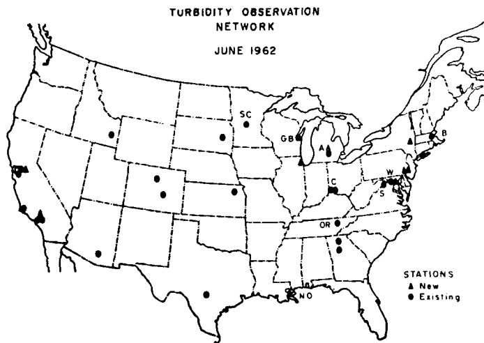
Fig. 2. Stations of the US turbidity network by 1962.
