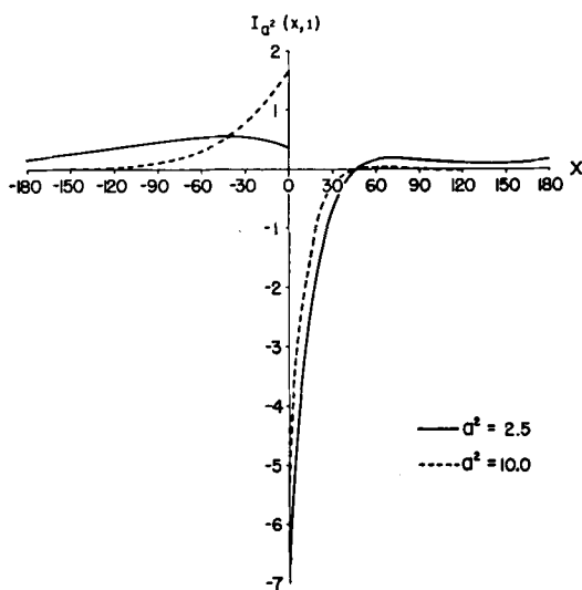
Fig. 5. The influence function I_a^2(x, 1) for a^2 = 2.5 and a^2 = 10 . This function represents the 24 hour height change of the 500 mb surface, relative to a co-ordinate system x traveling with the mean current, produced by a concentrated initial disturbance at x = 0 .
