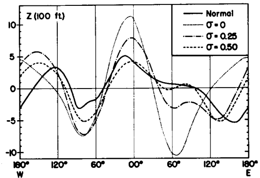
Fig. 4. Normal height profile of the 500 mb surface at 45° N for January together with computed stationary profiles for \sigma = 0 (no friction), for \sigma = 0.25 (moderate friction) and for \sigma = 0.50 (strong friction). For purposes of comparison the heights are represented as deviations from their respective means.
