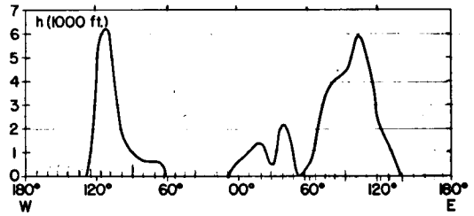
Fig. 3. Topographical profile at 45° N. The elevations represent the mean height of the earth's surface, averaged for the interval 40° N to 50° N, as a function of longitude.
