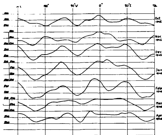
Fig. 2. Monthly mean profiles of the 500 mb level in middle latitudes ( 32.5^{\circ} — 62.5^{\circ} N).
