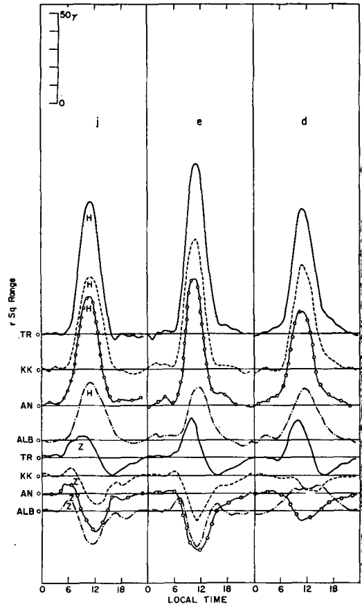
Fig. 2. Seasonal values of rSq(H) and rSq(Z) during the sunspot minimum. ( j = May to August; e = March, April, September and October; d = November to February).
