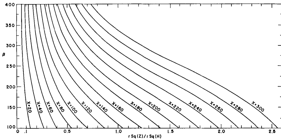
Fig. 3. Calculated rSq(Z)/rSq(H) against half-width \beta of the electrojet, for different distances ( X ) from magnetic equator.
