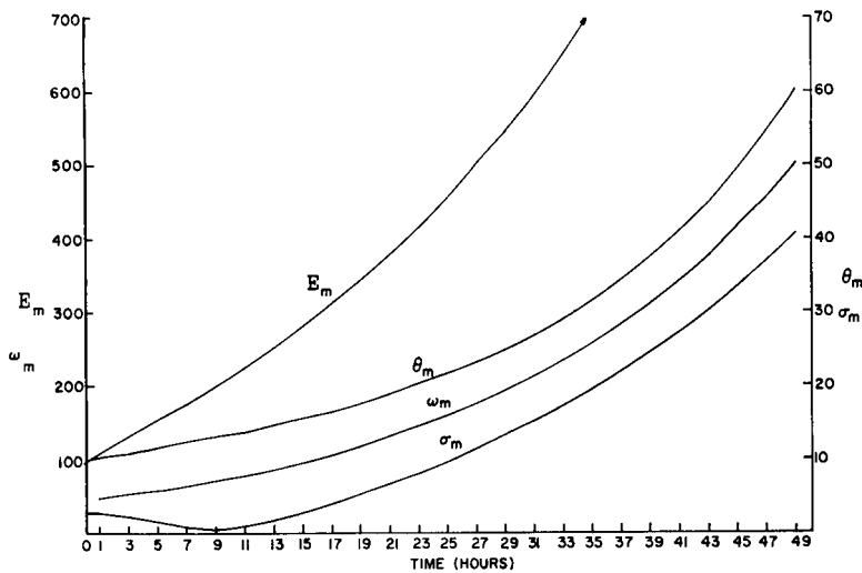
Fig. 3a. Amplitudes (ordinate), E_M (meters), \theta_M (degrees), \sigma_M (degrees) and \omega_M ( 10^{-4} mb sec ^{-1} ), of the stream, potential temperature, static stability and vertical velocity waves as functions of time (abscissa) for L = 4000 km, U^* = 15 m/s, \alpha = 90^\circ , \delta = 90^\circ , K = 100 ergs g ^{-1} °C ^{-1} sec ^{-1} , r = 2 .
