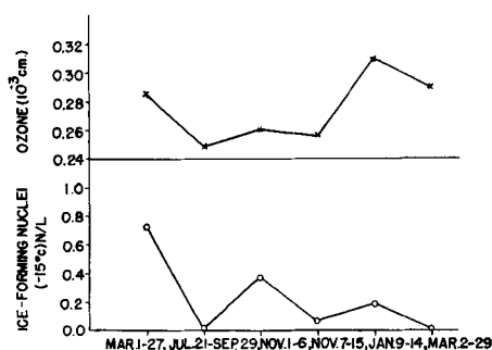
FIG. 6. Ice nuclei concentration and atmospheric ozone content (1962–63).
