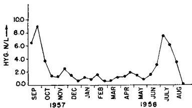
FIG. 1. Average half monthly concentration of giant hygroscopic nuclei (1957-58).
