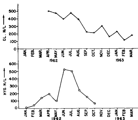
FIG. 2. Monthly mean concentration of hygroscopic (large size) and chloride aerosols (1962-63).
