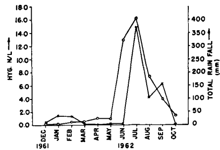
FIG. 3. Monthly mean concentration of giant hygroscopic aerosols (○) and total monthly rainfall (×) (measurements Dec. 1961 to Oct. 1962).
