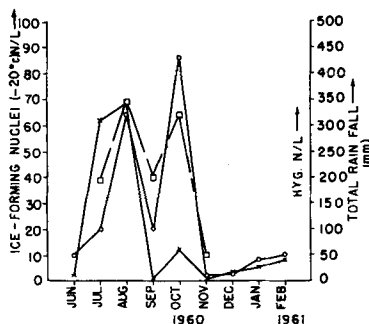
FIG. 4. Monthly mean concentration of ice-forming nuclei (○), large hygroscopic nuclei (□) and total monthly rainfall (×) (measurements 1960-61).
