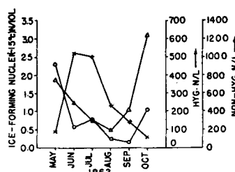
FIG. 5. Monthly mean concentration of ice-forming (○), large hygroscopic (×) and large non-hygroscopic aerosols (Δ), (measurements 1962).
