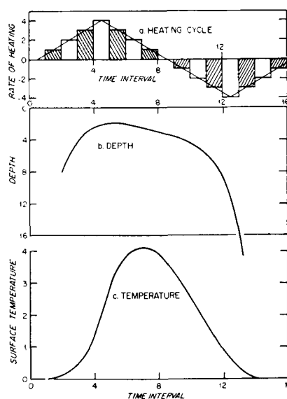
FIG. 7. Theoretical calculation of time-dependent surface layer behaviour, with constant stirring and an intermittent heat input. (a) The assumed saw-tooth heating function, and its approximation by steps. (b) Depth of the well-mixed surface layer at the end of each stirring interval. (c) The surface temperature at the end of each interval.
