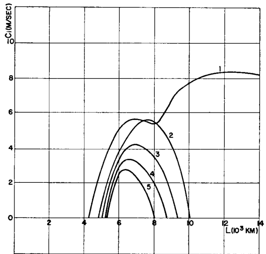
FIG. 11. Similar to figure 10 with N=7 (Fourier method).
