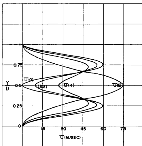
FIG. 17. Similar to figure 16, except that D = 6000 km and L = 4000 km.
