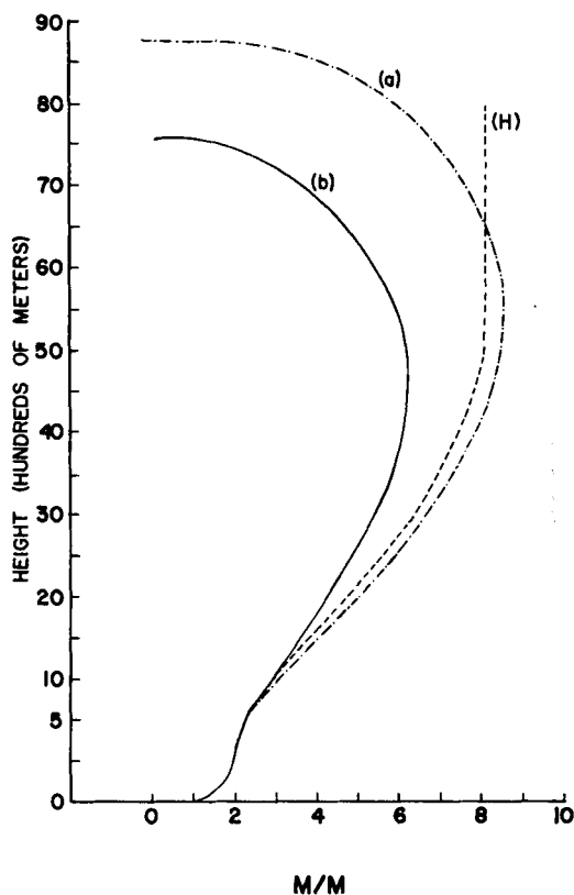
Figure 2. Fractional mass change M/M_0 as a function of height for Case (a), Case (b) and after HALTINER (1959).
