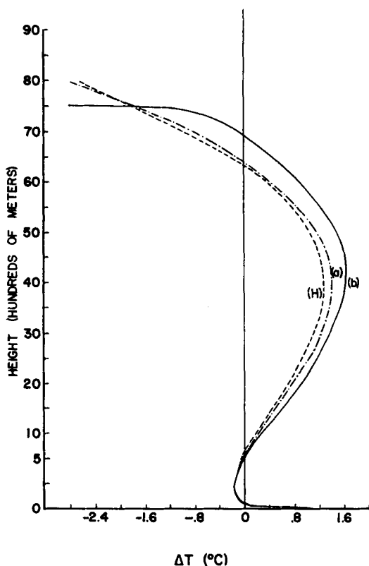
Figure 1. Temperature excess over environment as a function of height for Case (a), Case (b) and after HALTINER (1959).
