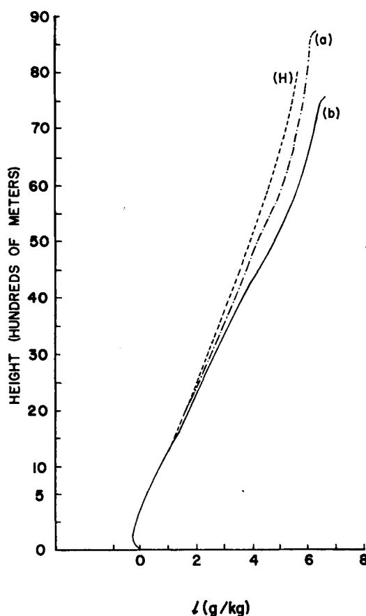
Figure 4. Liquid water content as a function of height for Case (a), Case (b) and after HALTNER (1959).
