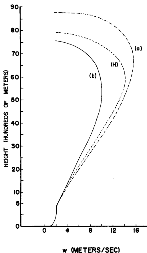
Figure 3. Vertical velocity as a function of height for Case (a), Case (b) and after HALTNER (1959).
