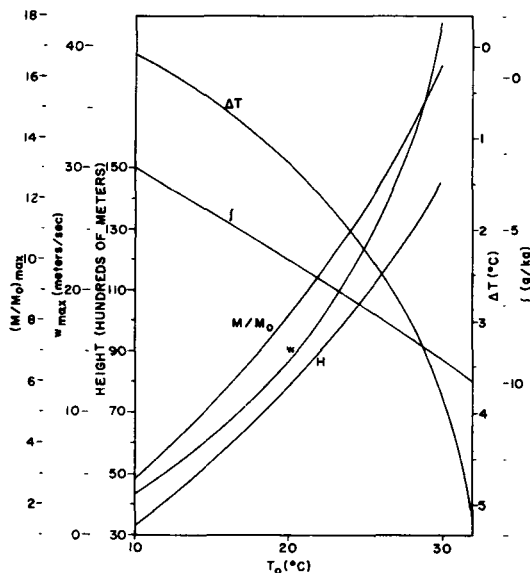
Figure 4. Cloud height H and maximum w , M/M_0 , l , and \Delta T as functions of initial temperature.
