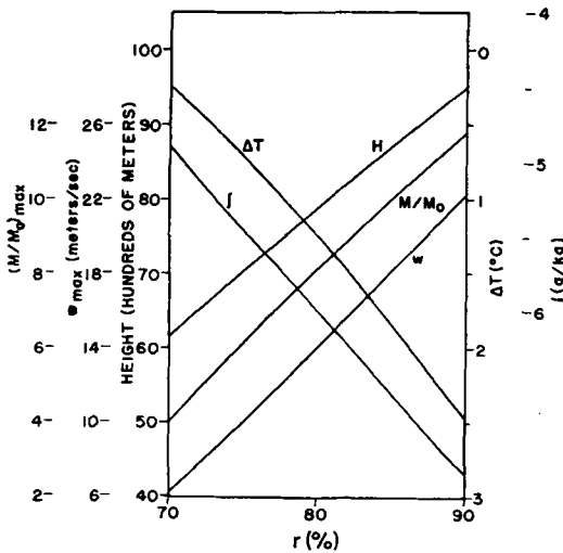
Figure 2: Cloud height H and maximum w , M/M_0 l and \Delta T as functions of environmental relative humidity r .
