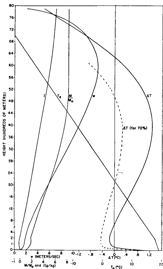
Figure 7. Similar to Fig. 1 except that k_2 = .0000025 \text{ cm}^{-1} .
