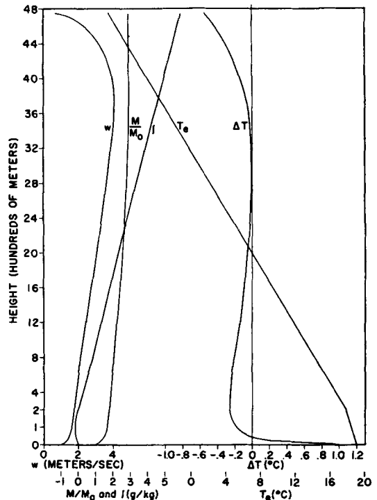
Figure 3. Similar to Fig. 1 except that \gamma_e = .6^\circ \text{C}/100 \text{ m} .
