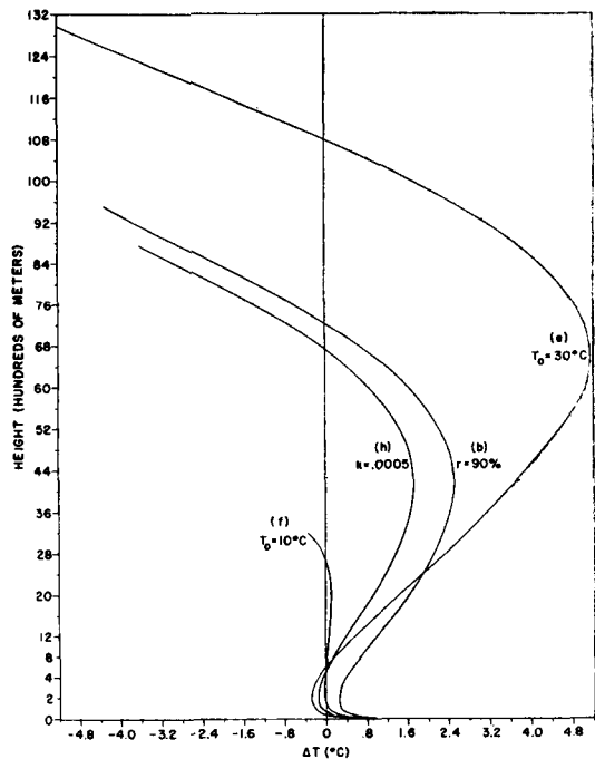
Figure 5. Temperature excess \Delta T = T - T_e of updraft over environment as a function of height for Cases (b), (e), (f) and (h).
