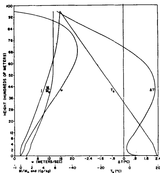
Figure 6. Similar to Fig. 1 except that w_0 = 2 meter/sec.
