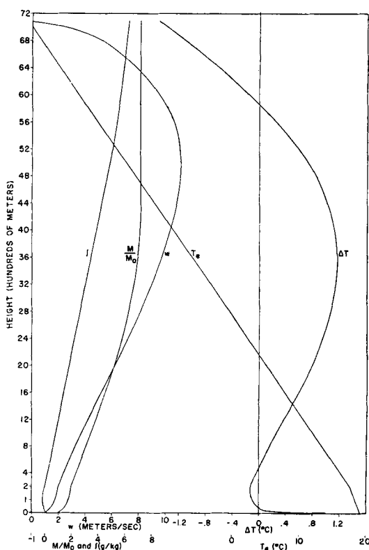
Figure 1. Vertical velocity w , fractional mass increase M/M_0 , liquid water content l , temperature excess over environment \Delta T and environment temperature T_e as functions of height for the convective current of Case (a), corresponding to \gamma_e = .7^\circ \text{C}/100 \text{ m} , r = 80\% , T_e = 20^\circ \text{C} , T_{e0} = 19^\circ \text{C} , w_0 = 1 \text{ mps} , k_1 = .001 \text{ sec}^{-1} . The dashed curve is \Delta T for Case (c), r = 70\% .
