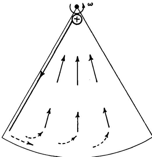
Fig. 3. Sketch of flow pattern expected with source \oplus at apex of sector, surface of fluid rising uniformly. (Dashed arrows are sketched in to indicate portions of flow not given by elementary theory but evidently required by continuity.)
