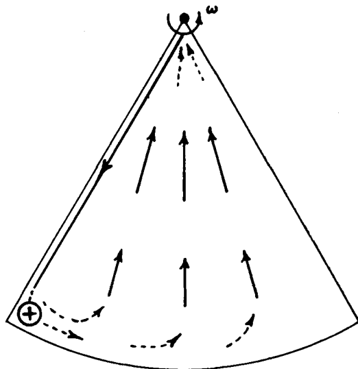
Fig. 4. Sketch of flow pattern expected with source \oplus at western edge of rim, surface of fluid rising uniformly.
