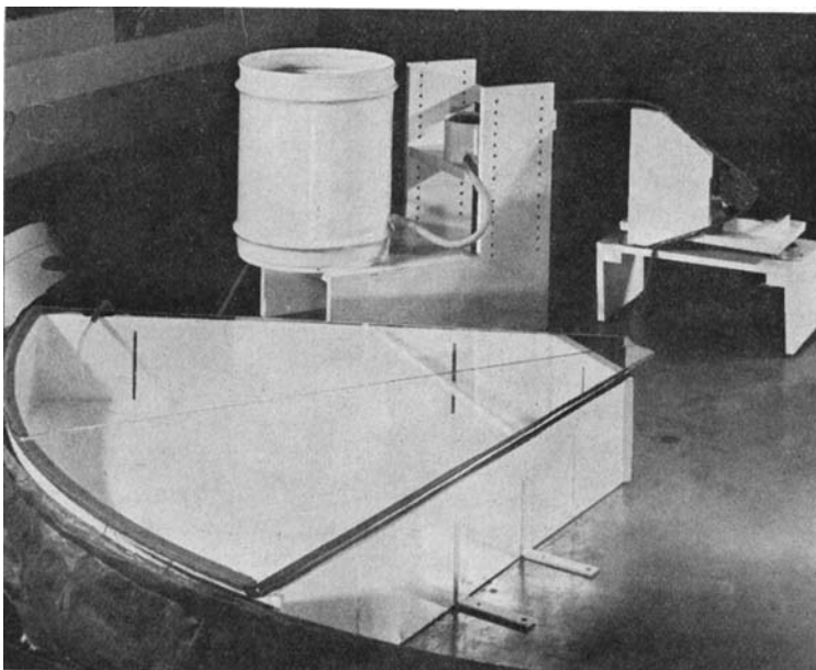
Fig. 6. A photograph of the rotating tank showing the 60^\circ sector with 1/4 -inch slots at various positions in the walls for the introduction or extraction of mass. When not in use the slots are sealed with tape. The glass cover prevents wind stress on the free surface of the water. A controlled flow rate is obtained by adjusting the level of the small can (with an overflow) into which water is pumped continuously. A constant head of water is thereby maintained in the large can containing the dyed source water.
