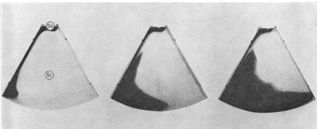
Fig. 8. Photographs at 20, 60, and 80 minutes with S_0 \approx 120 cc./min. The source was at the apex and there was no external sink (corresponding to Fig. 3).
