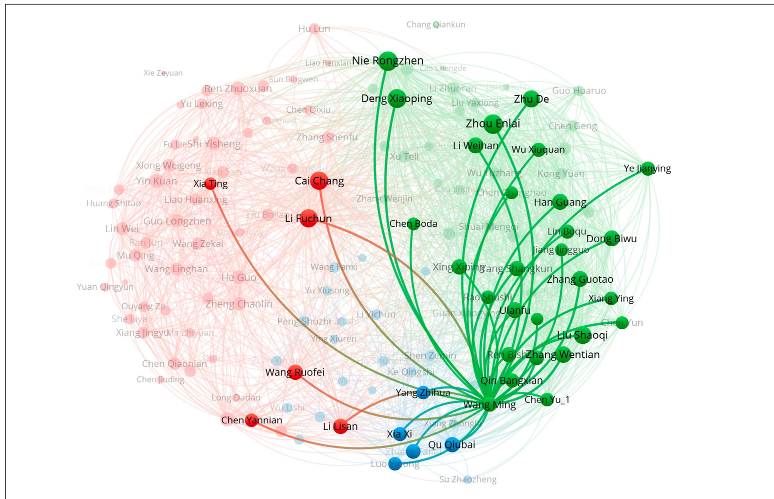
Fig. 12 Ego network for Wang Ming, pruned to 1,500 ties from the SRL dataset.
