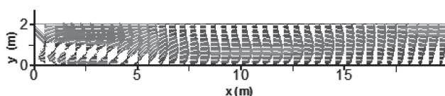
Fig. 10 Presentation of the recirculation zone.
