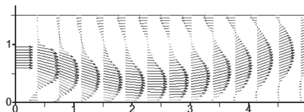
Fig. 8 Presentation of the recirculation zone.
