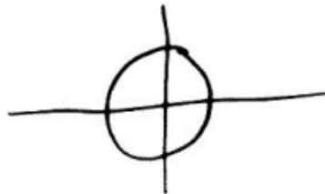
FIGURE 2. The 340 cipher.
