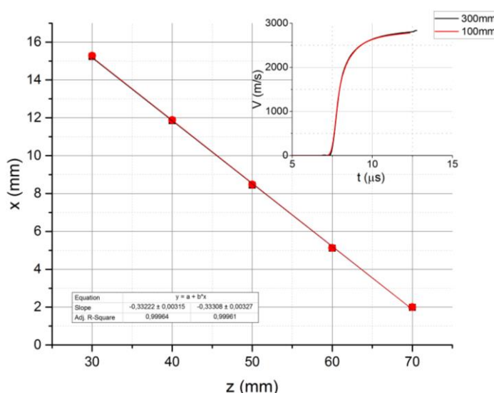
Fig. 5. Gurney speed and armature wall deformation for armature length of 100 mm (red) and 300 mm (black) at 10 \mu s after detonation initiation; steeper angle equals higher velocity of detonation
