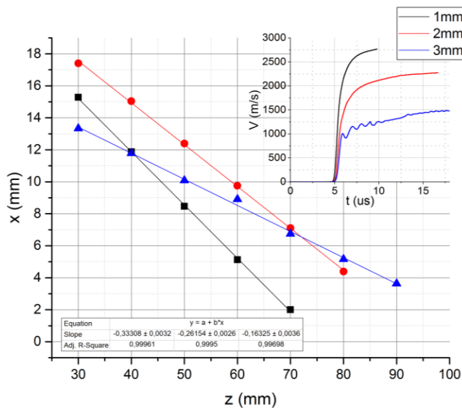
Fig. 6. Gurney speed and armature wall deformation for armature wall thickness of 1 mm (black), 2 mm (red) and 3 mm (blue); armature wall deformation at 10 \mu s (1 mm), 13 \mu s (2 mm) and 15 \mu s (3mm) after detonation initiation; steeper angle equals higher velocity of detonation
