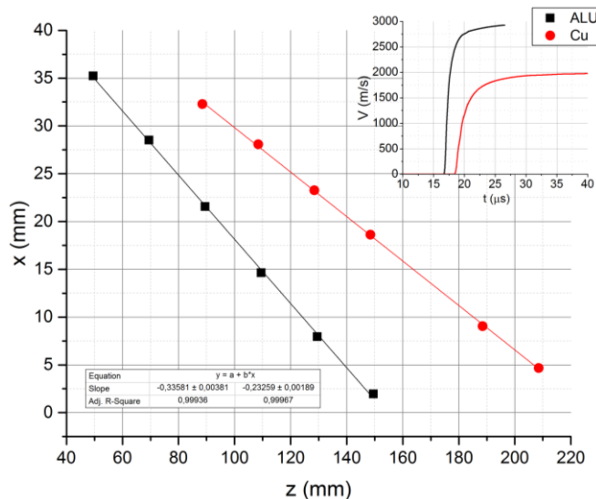
Fig. 4. Gurney speed and armature wall deformation for copper (red) and aluminum (black); armature wall deformation at 20 μs (aluminum) and 30 μs (copper) after detonation initiation; steeper angle equals higher velocity of detonation
