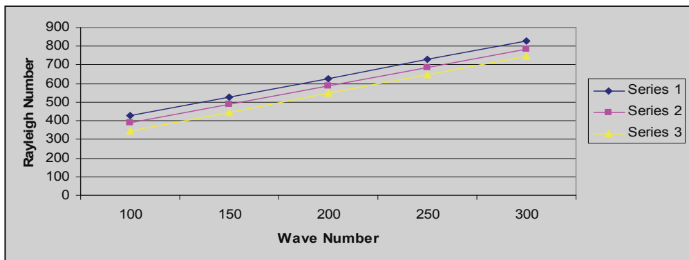
Fig. 2. The stabilizing effect of stable solute gradient S_2
