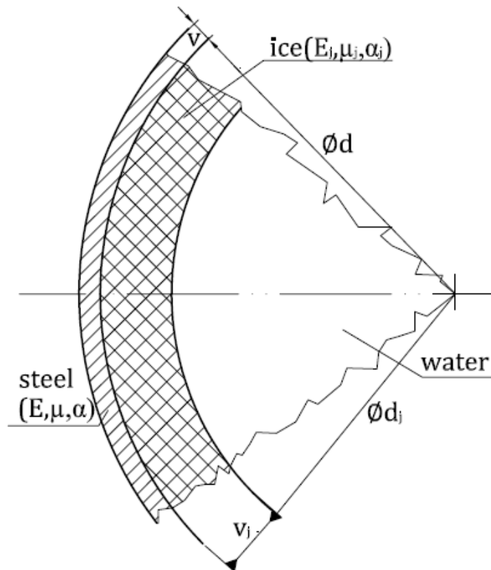
Fig. 11 Cross section of hydroglobe with ice layer
