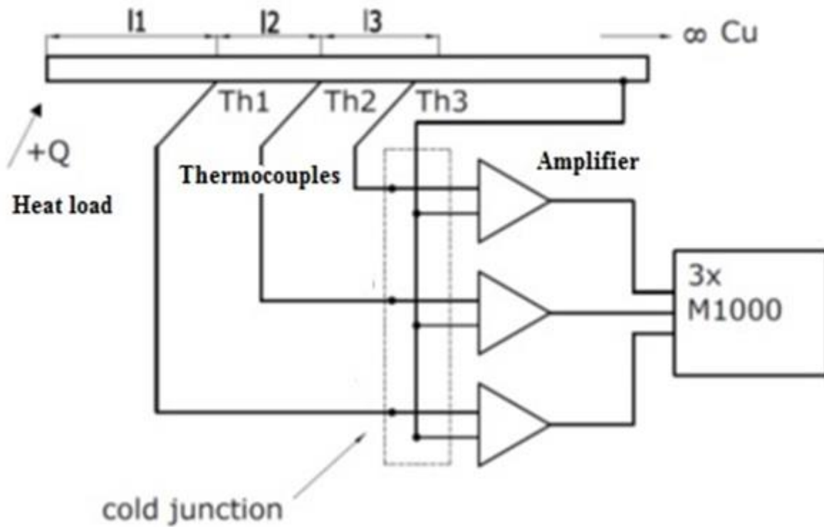
Fig. 8 Test setup for relaxation time
