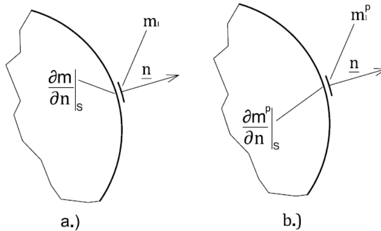
Fig. 5 Boundary condition for moisture diffusion a.) moisture concentration b.) moisture potential
