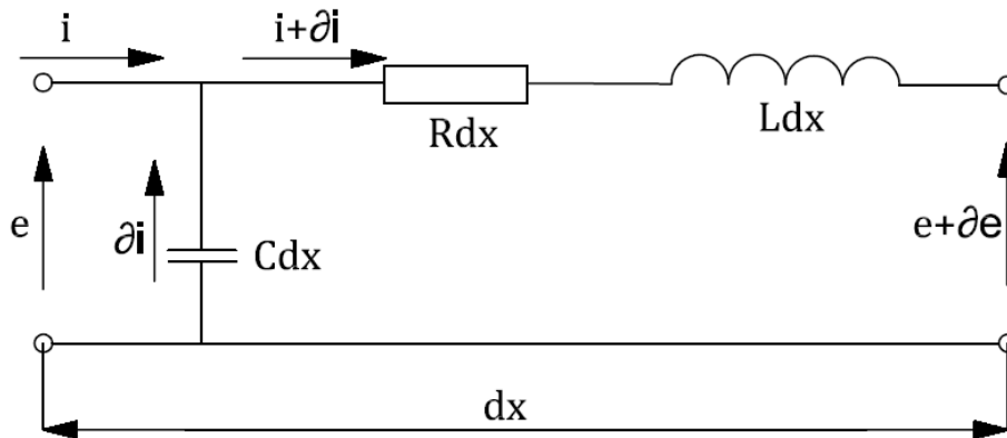
Fig. 2 Elementary circuit for heat conduction or moisture diffusion problem with second sound
