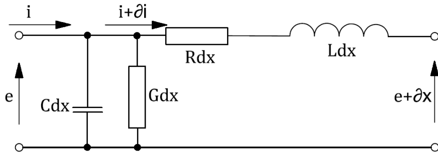
Fig. 1 Elementary circuit for coupled thermoelastic problem
