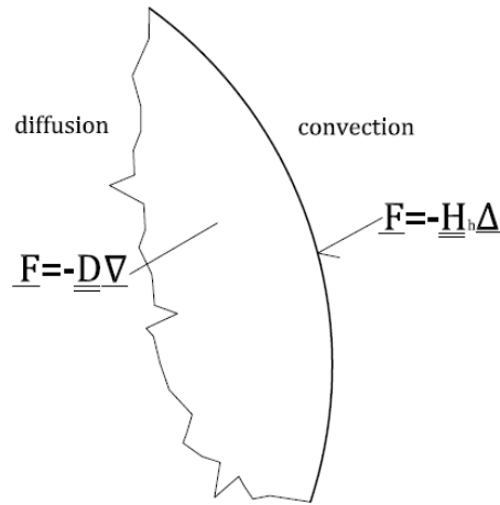
Fig. 6 Boundary condition for cross-coupled heat and moisture diffusion
