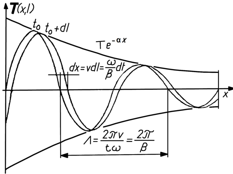
Fig. 7/a Temperature T (or moisture) vs. location, x
