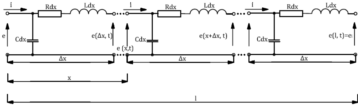
Fig. 4 Electrical model for for heat conduction or moisture diffusion problem with second sound
