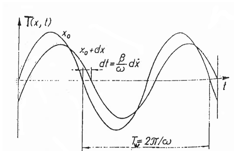
Fig. 7/b Temperature T (or moisture) vs. time, t
