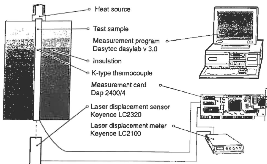
Fig. 10 Experimental setup for measure of diffusivity
