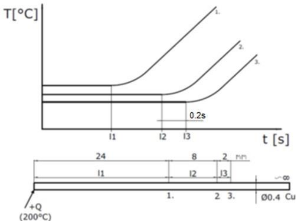
Fig. 9 Experimental results on relaxation time
