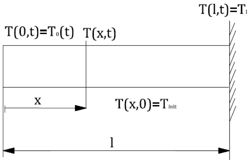
Fig. 2 Elementary circuit for heat conduction or moisture diffusion problem with second sound
