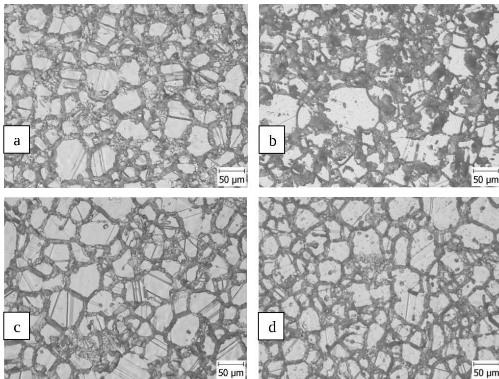
Fig. 2 Microstructure of steel P560 after corrosion tests under conditions: a) 750 °C/30min; b) 750 °C/10 hrs.; c) 900 °C/30 min.; d) 900 °C/10 hrs.
