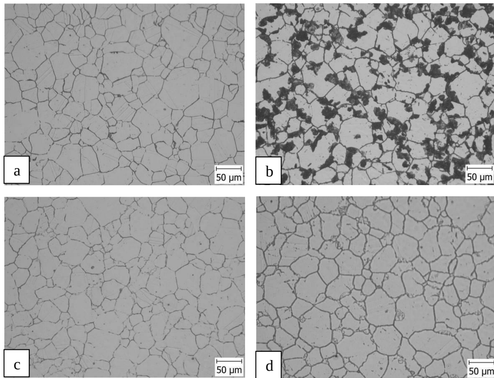
Fig. 1 Microstructure of the steel after isothermal annealing under conditions a) 750 °C/30 min; b) 750 °C/10 hrs.; c) 900 °C/30 min.; d) 900 °C/10 hrs.
