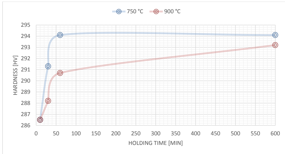
Fig. 3 Dependence of steel hardness on holding time before and after heat treatment
