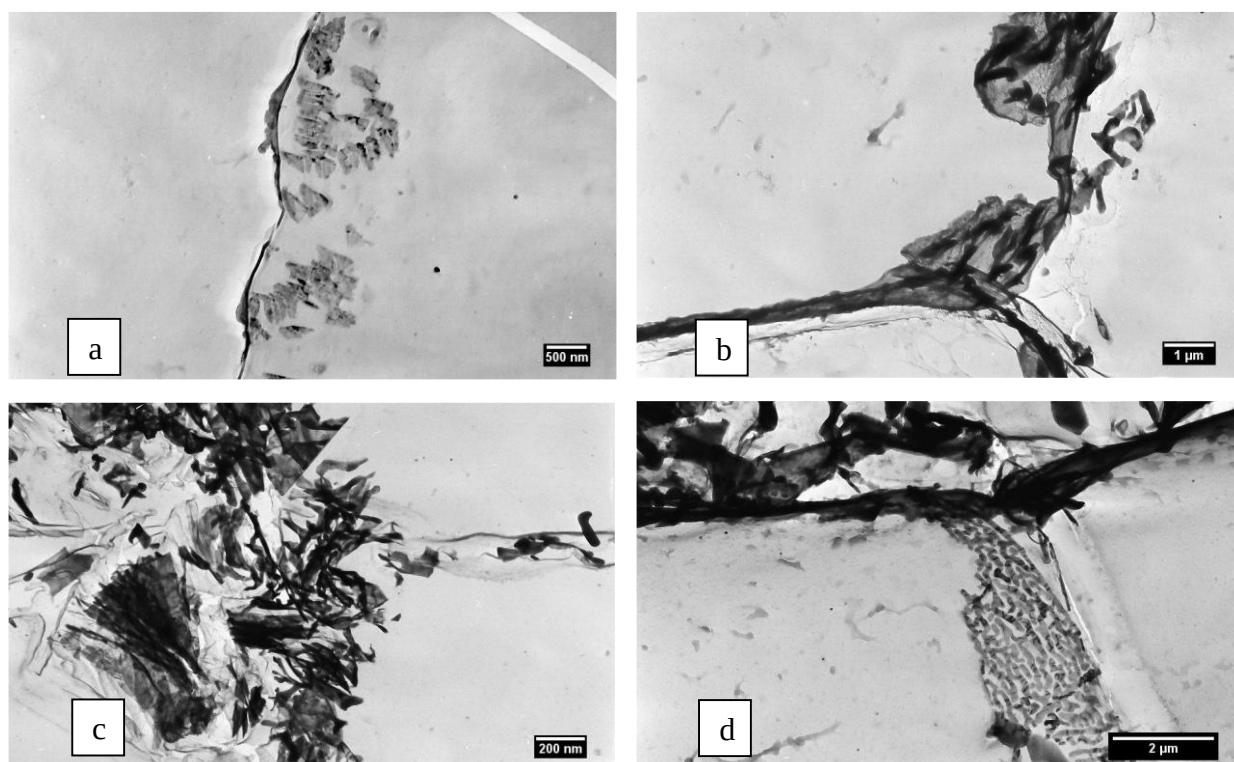
Fig. 4 The grain boundaries observed by transmission electron microscope, steel annealed at 750 °C for holding time of a) 10 min.; b) 30 min.; c) 1 hr.; d) 10 hrs.
