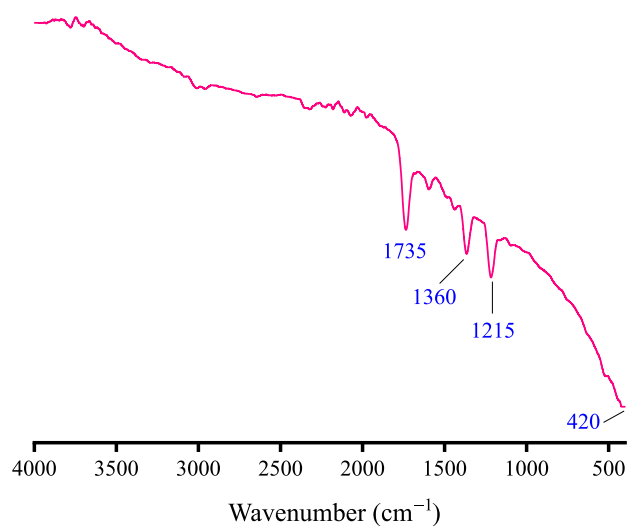
Figure 8. The IR spectrum of the RuO 2 material
