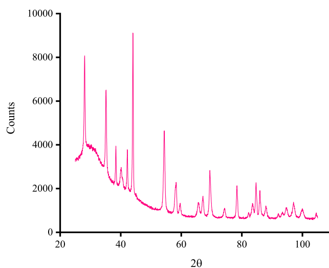
Figure 9. The XRD diffractogram of the RuO 2 material
