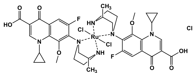
Figure 7. Proposed chemical structure of the synthesized complex; [\text{Ru}(\text{L})_2(\text{Cl})_2]\text{Cl}
