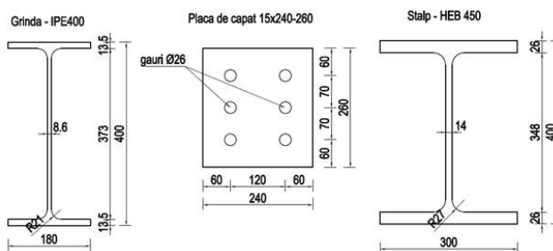
Fig. 4 Components of the Verified Joint
