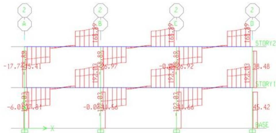
Fig. 2 Shear Force Diagram Results
