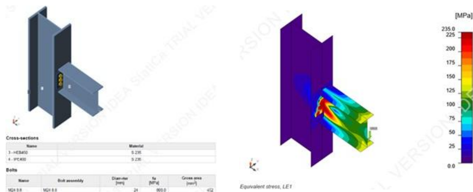
Fig. 5 The Joint Introduced in the IDEA StatiCa Program; Stress Distribution in the Joint
