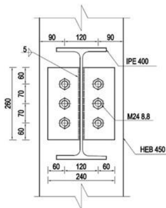
Fig. 3 Calculated Joint
