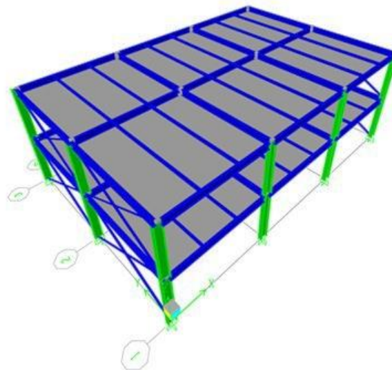
Fig.1 The metal structure studied
