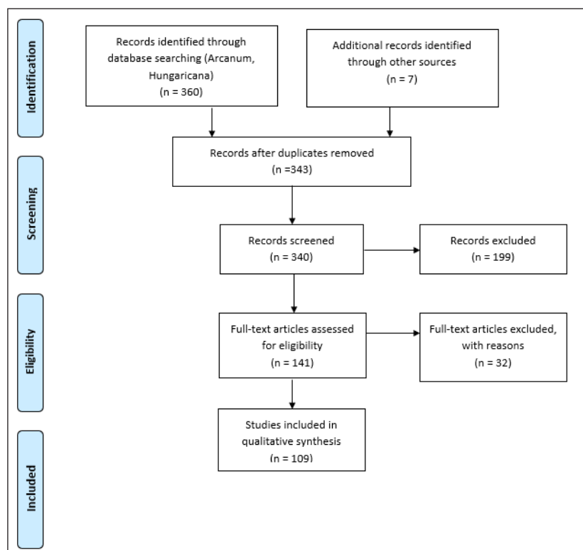
Figure 2. PRISMA flowchart
