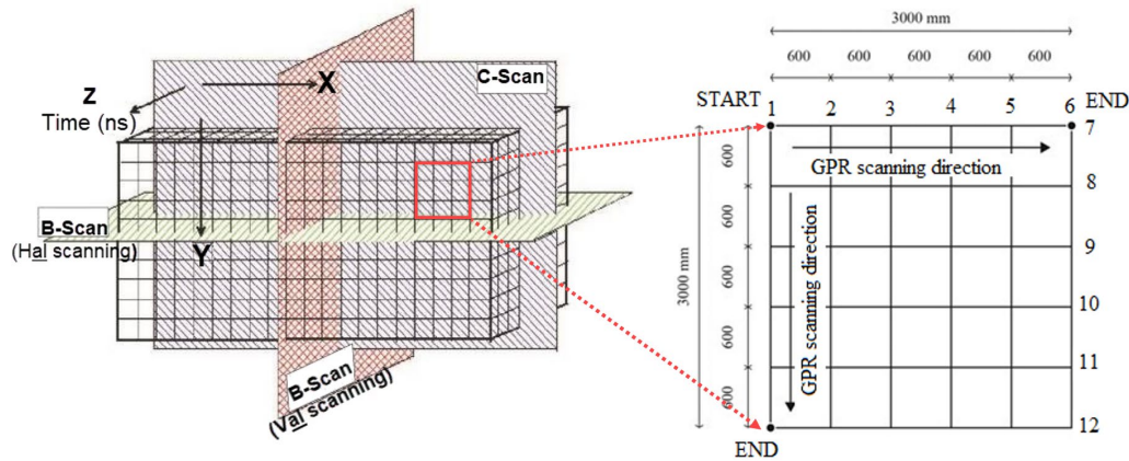
Figure 12 – Illustration of the grid mark scheme of the mock-up wall and the scanning direction.
