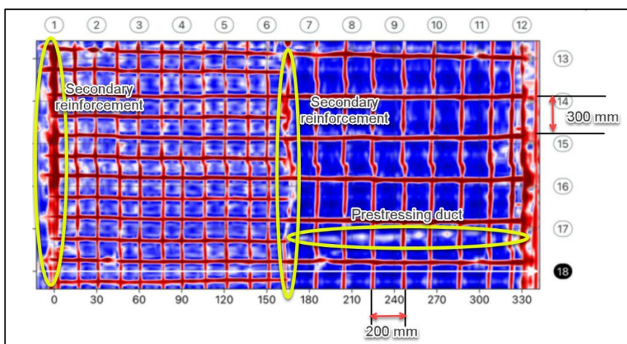
Figure 16 – C-Scan of the near-surface reinforcement of the southern side using GPR1 device.
