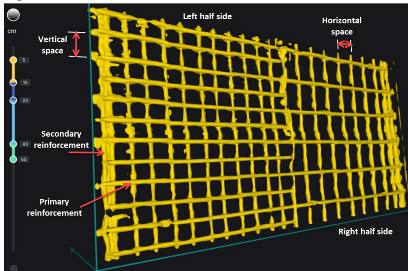
Figure 15 – Representation of the near-surface reinforcement of the southern face using GPR1 device.
