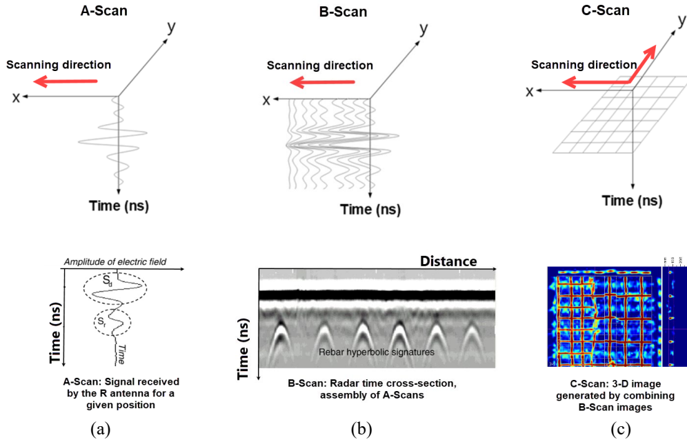
Figure 3 – Measurement principle for GPR. (a) A-scan is the signal of the receiving antenna for a given position, (b) B-scan is the assembly of A-scans and (c) C-scan is the 3-D image which is generated by combining simultaneous B-scan images on the XY plane [8], [9].
