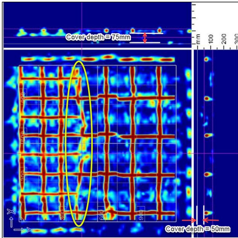
Figure 19 – Representation of the vertical middle part of the southern side using GPR2 device.
