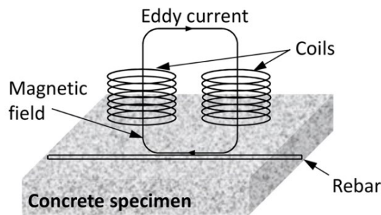
Figure 1 – Illustration of the concrete cover meter operation principle using eddy current.
