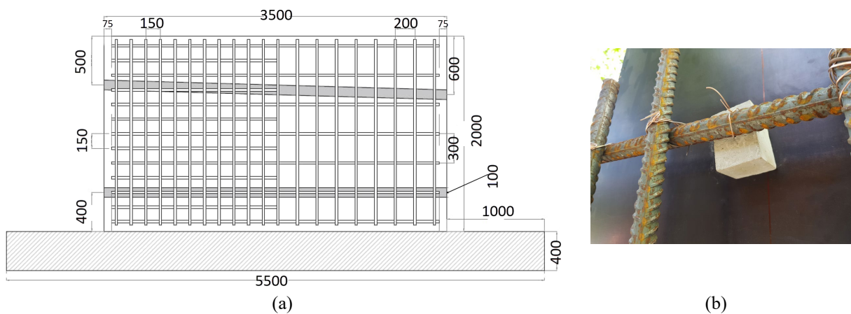
Figure 7 – (a) Frontal view of the mock-up wall with its reinforcement and (b) embedded 50 mm concrete block for indicating the actual cover thickness of the reinforcement bars.
