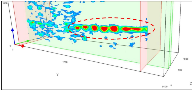
Figure 20 – Visual representation of the lower tendon strand using the UPE device.
