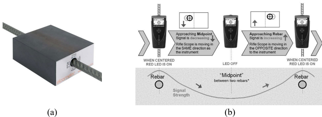
Figure 11 – Concrete cover meter: (a) the calibration test block and (b) distinguishing between a rebar and a mid-point using cover meter [16].
