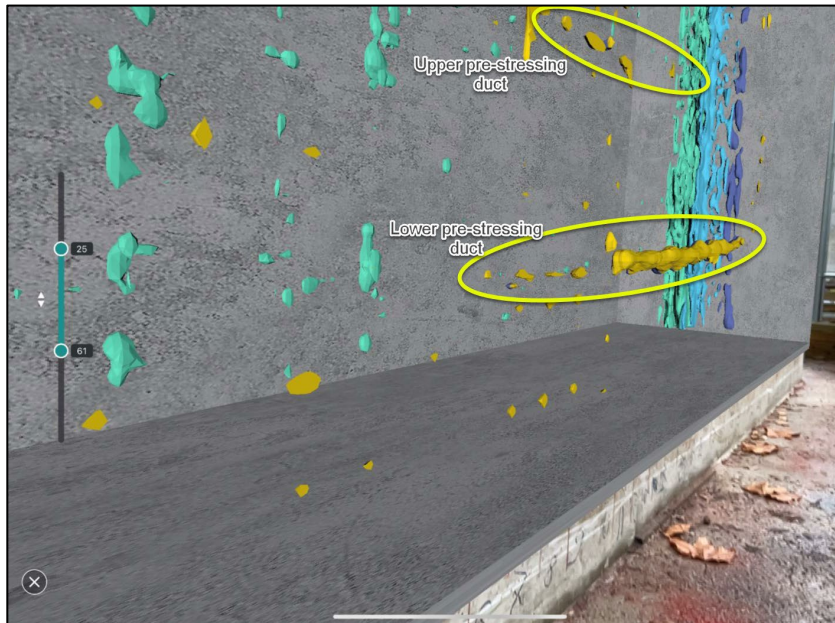
Figure 17 – Visual representation of the tendon strand on the southern side as an Augmented Reality (AR) view on the surface of the real structure using GPR1 device.
