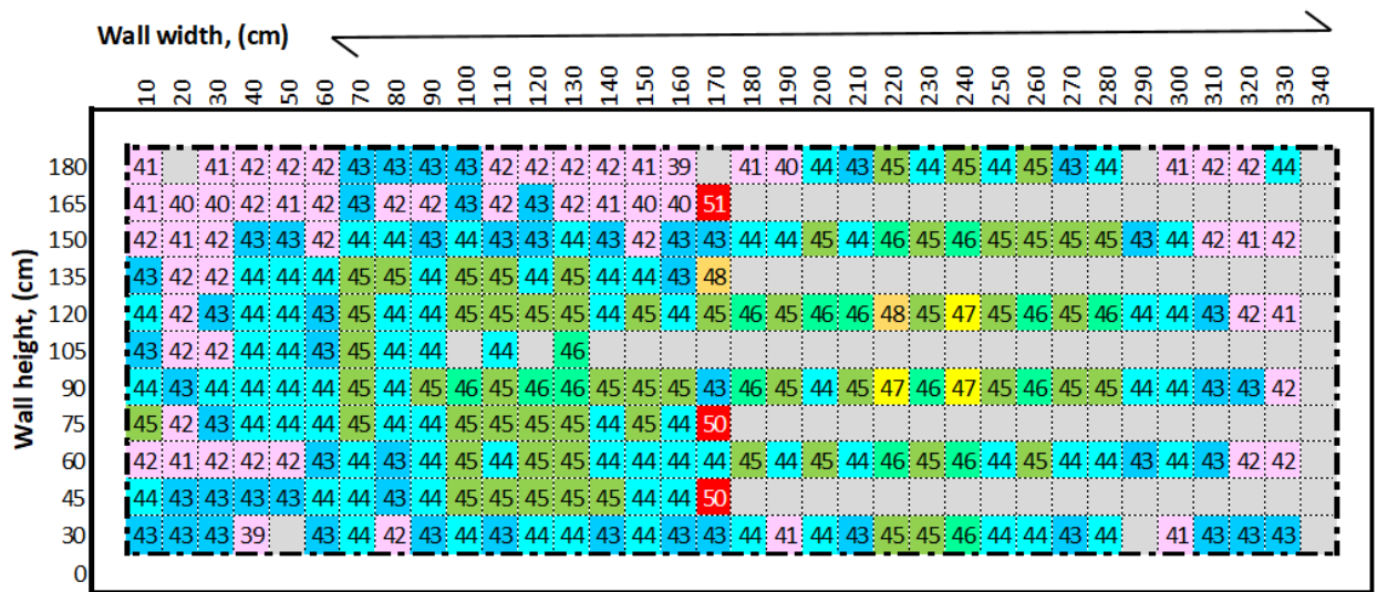
Figure 13 – Concrete cover thickness scanned for horizontal reinforcement on the south face of the wall).
