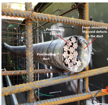
Figure 10 – Location of the void defects in the pre-stressed tendon ducts.
