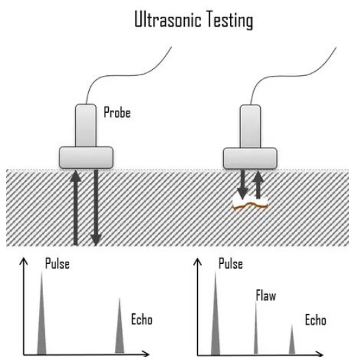
Figure 4 – Schematic diagram of the ultrasonic testing.
