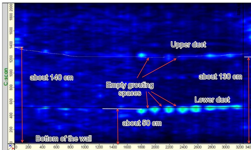
Figure 21 – Visual representation of the tendon strand using the UPE device compared to Figure 18.
