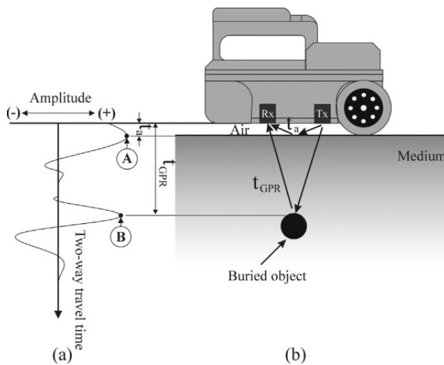
Figure 2 – Illustration of a GPR system and reflected signal from a buried object: (a) waveform, (b) reflection paths of radio wave [5] and [6].
