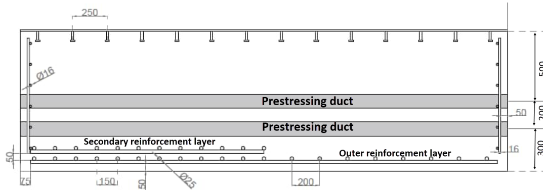
Figure 8 – Plan view of the mock-up main wall reinforcement.
