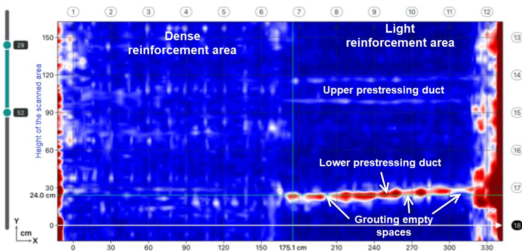
Figure 18 – Visual representation (C-Scan) of the tendon strand on the southern side using GPR1 device at the depth of 29 - 52 cm from the surface, compared to Figure 15.
