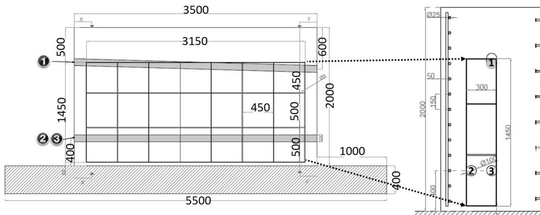
Figure 9 – Location of the pre-stressed tendon ducts, side views.
