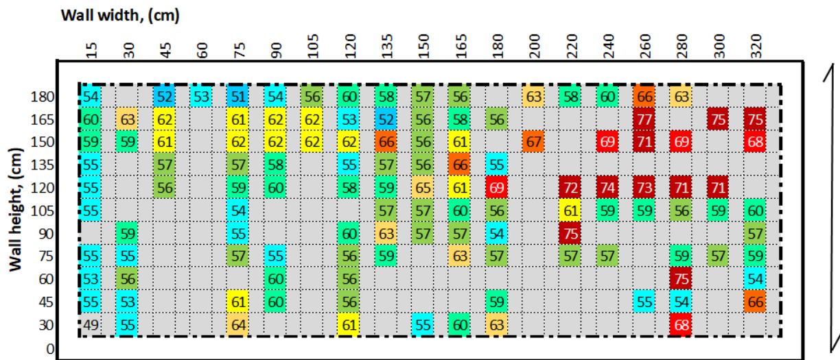
Figure 14 – Concrete cover depth (south face, vertical reinforcement scanning).
