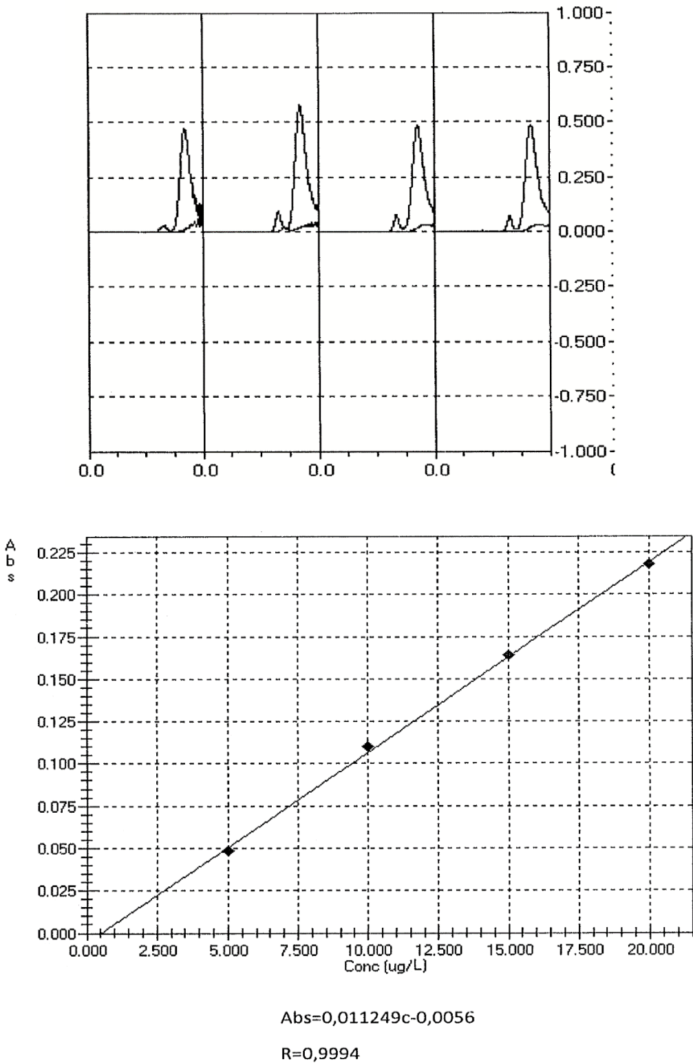
Fig. 1: Calibration curve for Cu measurement.
