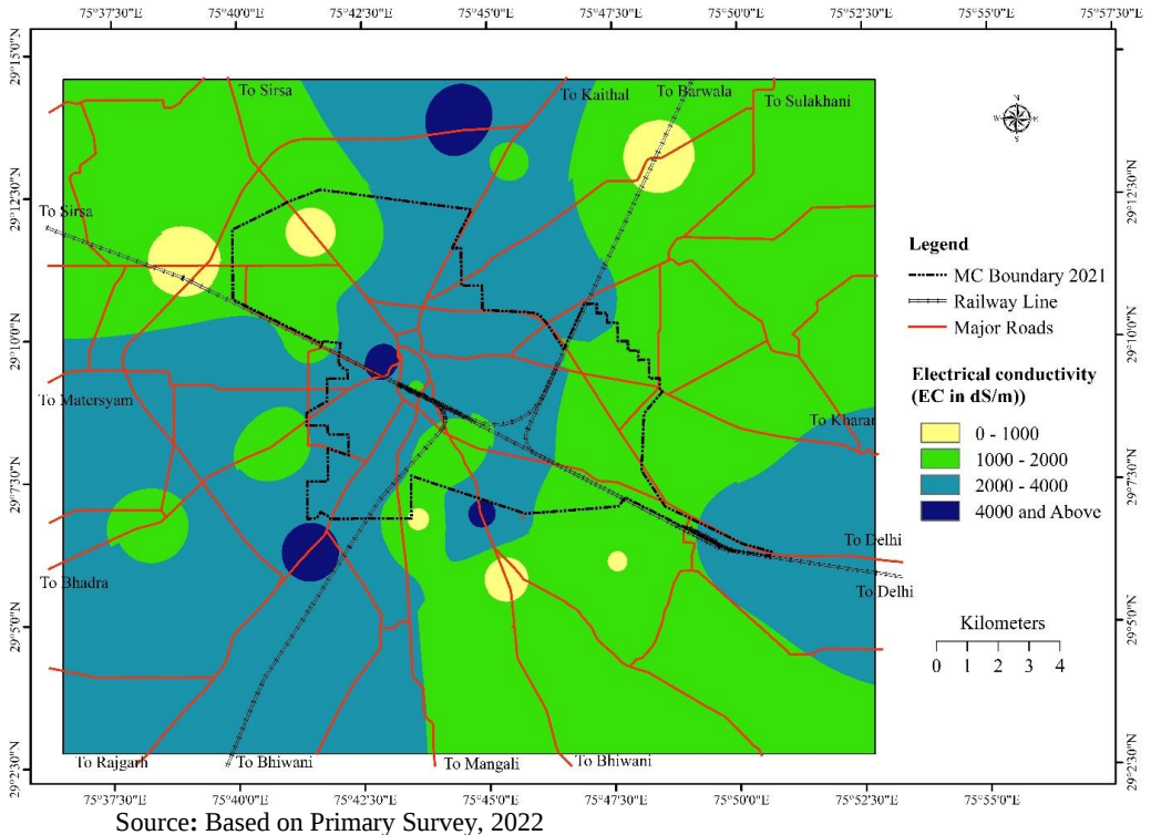
Fig. 4: Ground Water Quality of Hisar City and Its Periphery
