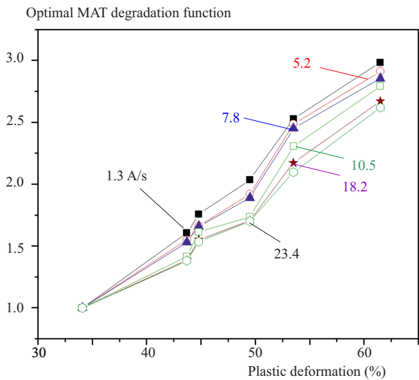
Fig. 2. The optimal descriptors, determined for the series of the cold rolled austenitic stainless steel plates, at different speeds of the magnetizing current
