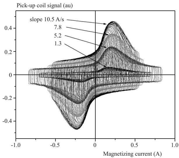
Fig. 1. Measured signal of the pick-up coil as a function of magnetizing current for different speeds of magnetization, in the case of the most ferromagnetic piece of samples
