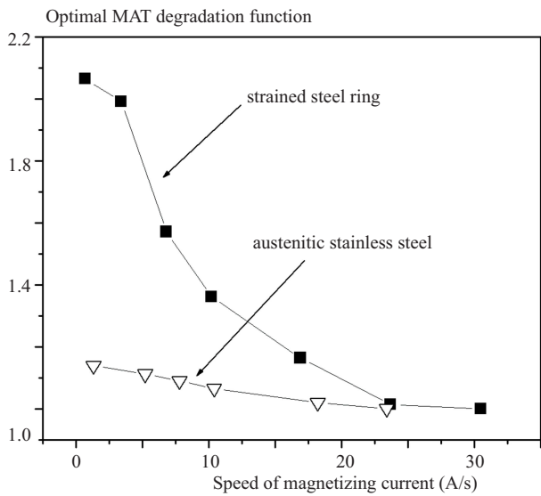
Fig. 3. Optimal MAT descriptors of the austenitic stainless steel and of a plastically deformed steel of ref.[6] as functions of the speed of magnetizing current
