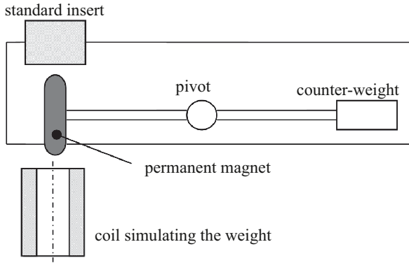
Fig. 1. Setup of the low- \mu permeability indicator with a cylindrical coil
