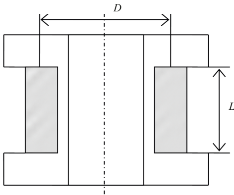
Fig. 2. A cylindrical coil for simulating the weights
