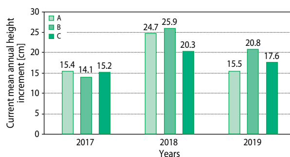
Figure 2. Current mean annual height increment (cm) of pedunculate oak ( Q. robur ) trees in stands established in 2012 using container-grown seedlings (A), three-year-old bare-root seedlings (B), and direct acorn sowing (C)
