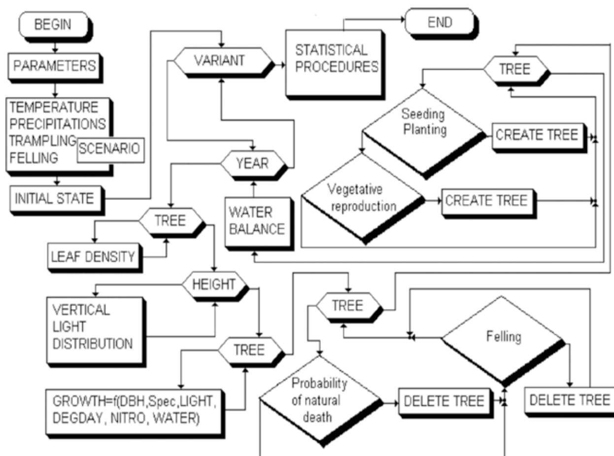
Figure 3. Block diagram of the UFB model (Kozak et al. 2023), the full term of DBH given in the figure: diameter at breast height
