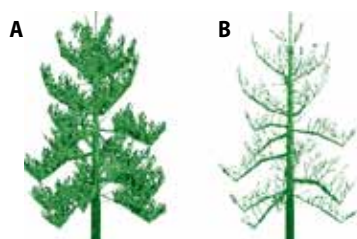
Figure 4. Percentage of drying of assimilation apparatus of Scots pine as depicted in the UFB model: a) 0%, b) 100%
