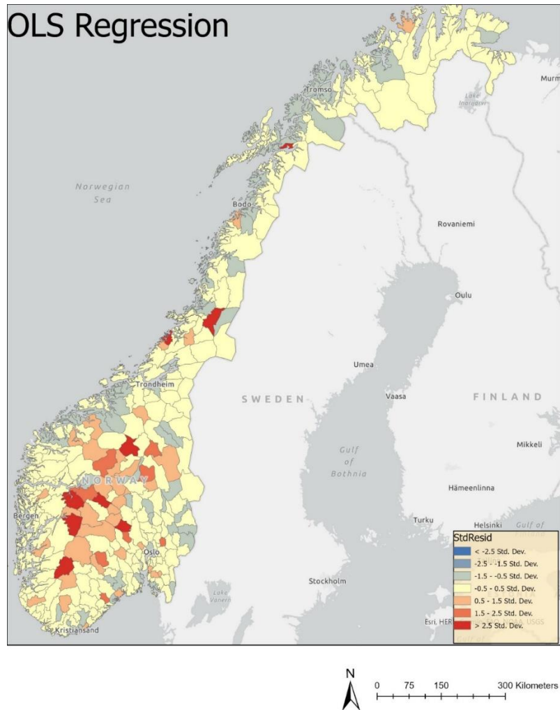
Figure 8: OLS regression
