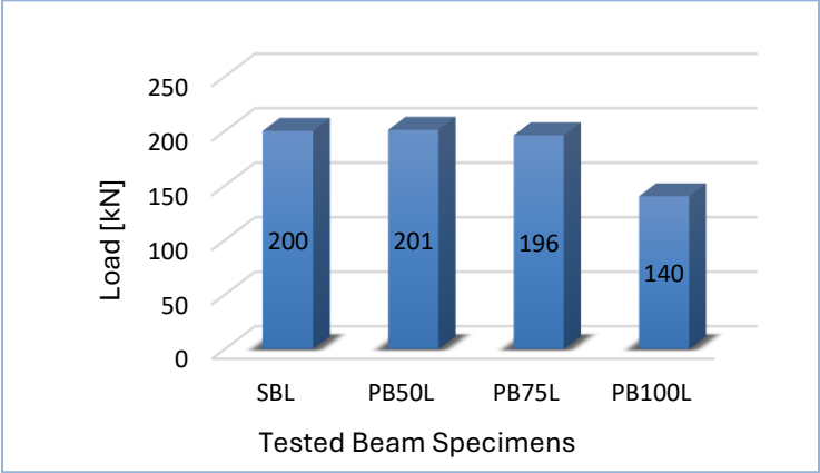
Figure 7: Ultimate loads of all beams
