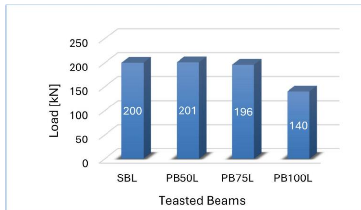
Figure 7: Ultimate loads of all beams
