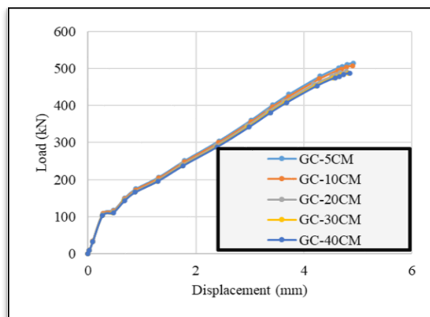
Fig. 17: load-displacement curve numerical series.
