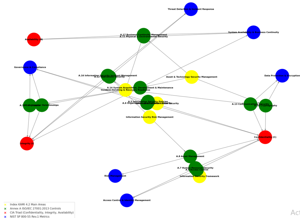
Fig. 3. Alignment relationship diagram between the CIA Triad and the main areas of the KAMI Index Version 4.2, ISO/IEC 27001:2013, and NIST SP 800-55 Rev.1
