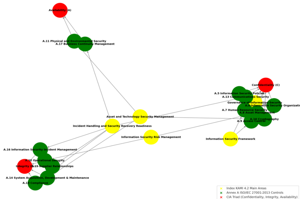
Fig. 2. Alignment relationship diagram between the CIA Triad and the main areas of the KAMI Index Version 4.2 and ISO/IEC 27001:2013
