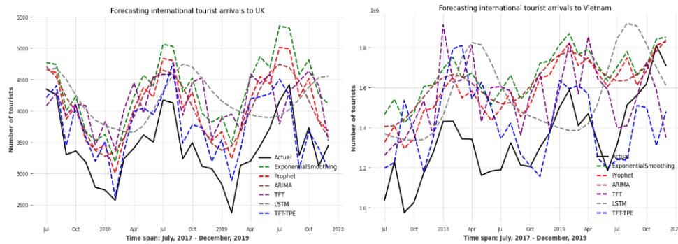
Fig. 7. Comparison of forecast results and actual international arrivals in the UK and Vietnam (from December 2017 to December 2019)
