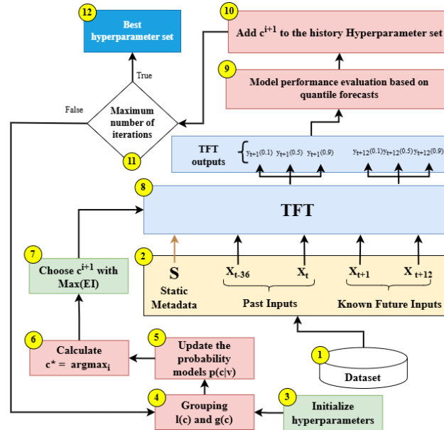
Fig. 2. The proposed TFT-TPE integrated model
