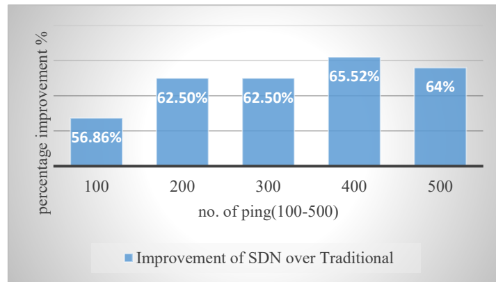
Fig. 8. Percentage improvement of SDN over Traditional regarding Average RTT
