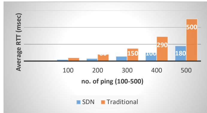
Fig. 7. Average RTT vs No of pings
