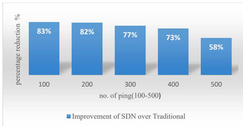
Fig. 6. Percentage reduction of SDN over Traditional regarding the Total No Pkts_dropped
