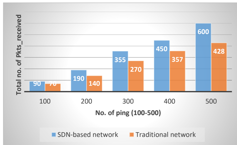
Fig. 3. Total No of Pkts_received vs No of ping
