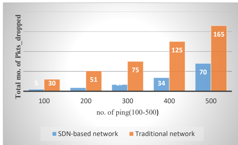
Fig. 5. Total No of Pkts_dropped vs the number of ping
