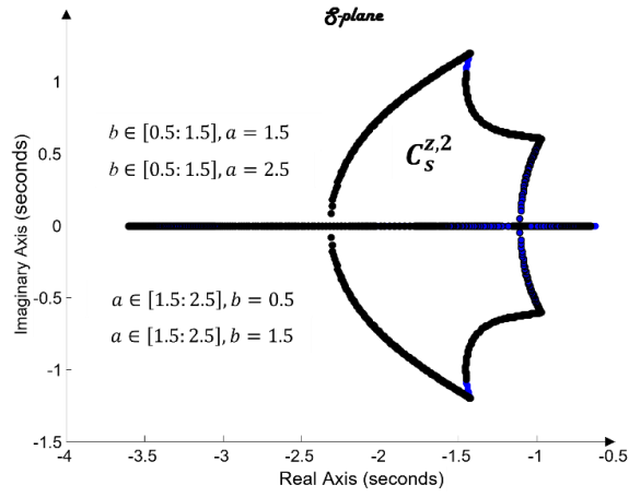
Fig. 6. Root contour for k_e = 2
