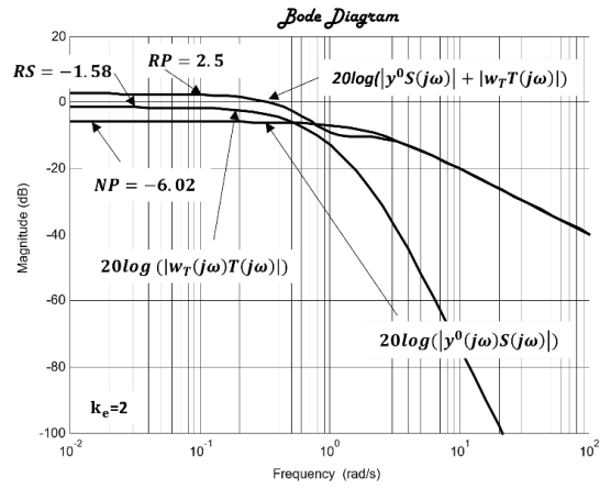
Fig. 7. Bode diagram of nominal performance, robust stability, robust performance, k_e = 2
