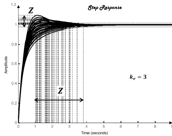
Fig. 11. Transient performance of control systems (uncertainty parameters), k_e = 3
