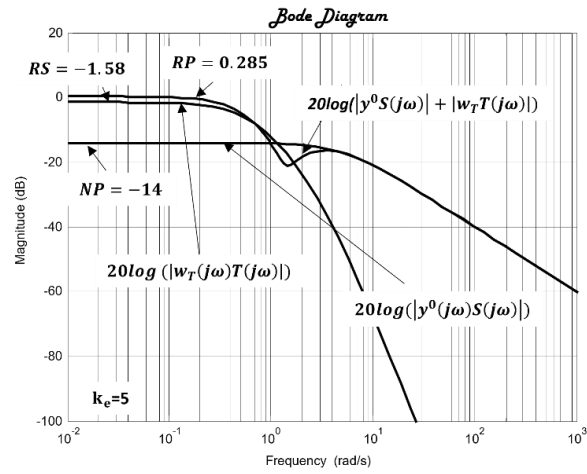
Fig. 13. Bode diagram of nominal performance, robust stability, robust performance, k_e = 5
