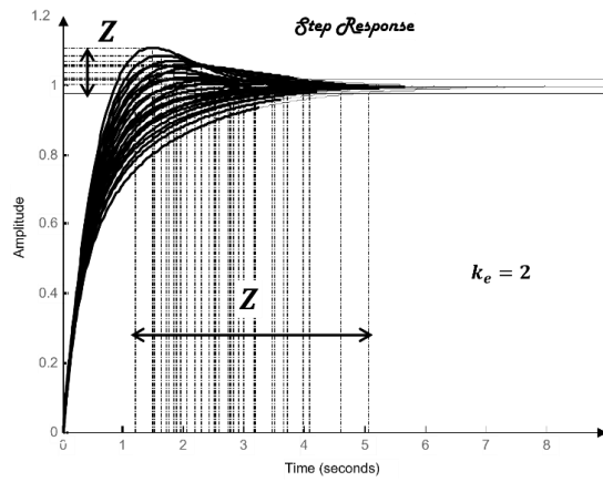
Fig. 8. Transient performance of control systems (uncertainty parameters), k_e = 2
