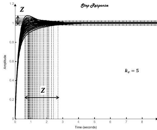
Fig. 14. Transient performance of control systems (uncertainty parameters), k_e = 5
