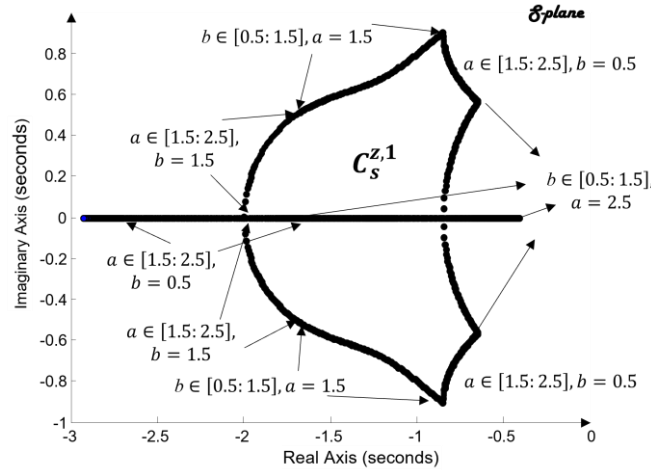
Fig. 4. Root contour of closed loop system, k_e = 1
