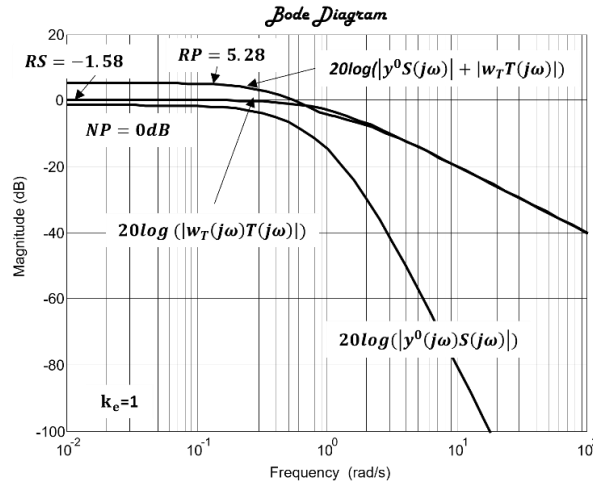
Fig. 5. Bode diagram of nominal performance, robust stability, robust performance, k_e = 1
