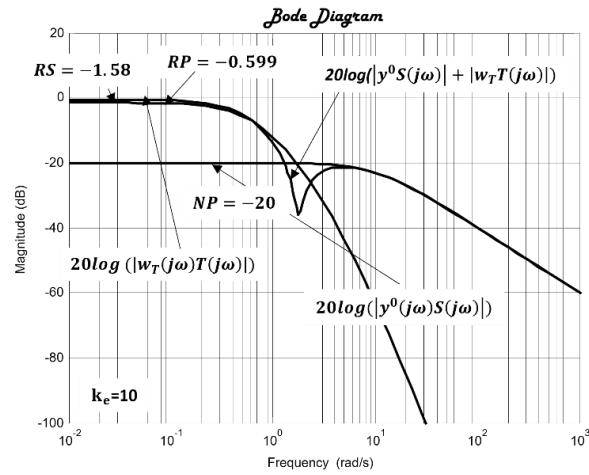
Fig. 16. Bode diagram of nominal performance, robust stability, robust performance, k_e = 10
