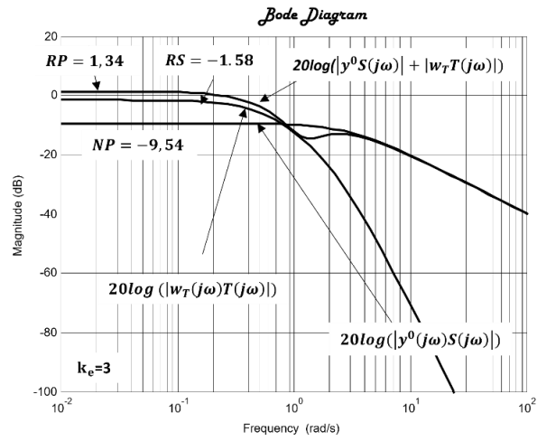
Fig. 10. Bode diagram of nominal performance, robust stability, robust performance, k_e = 3
