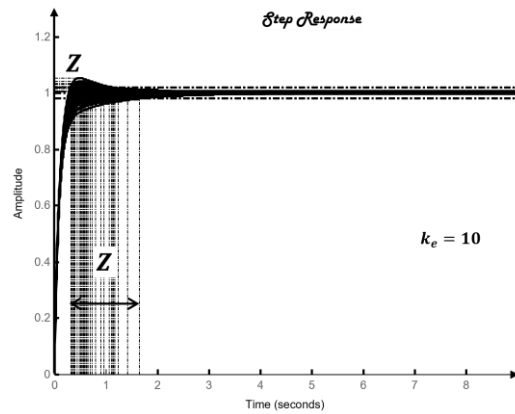
Fig. 17. Transient performance of control systems (uncertainty parameters), k_e = 10
