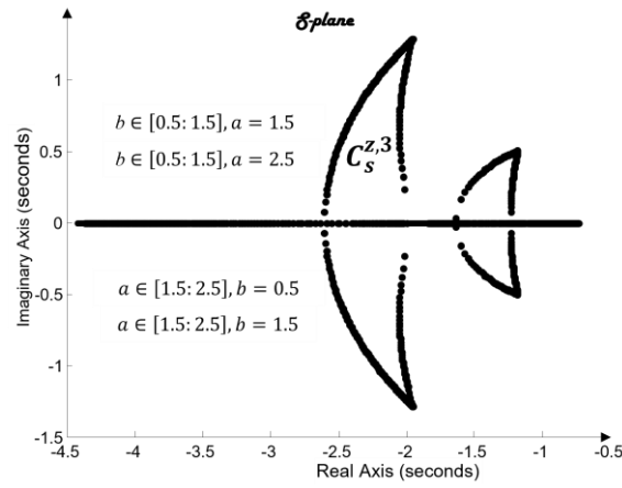
Fig. 9. Root contour for k_e = 3
