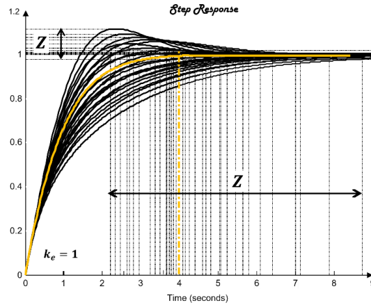
Fig. 3. Transient performance of control systems (uncertainty parameters, k_e = 1 )
