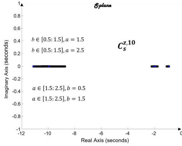
Fig. 15. Root contour, k_e = 10
