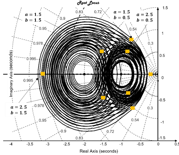
Fig. 2. Root Locus of control systems (uncertainty parameters)
