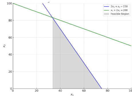
Fig. 1. Feasible region of economic resource allocation
