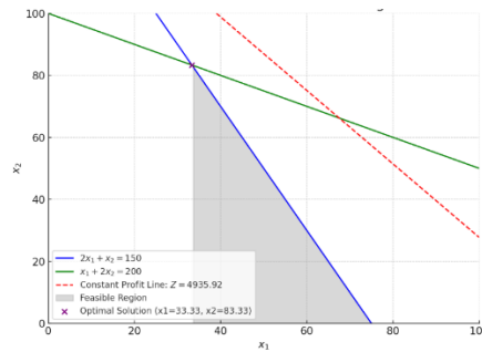
Fig. 2. Maximum profit line and feasible region
