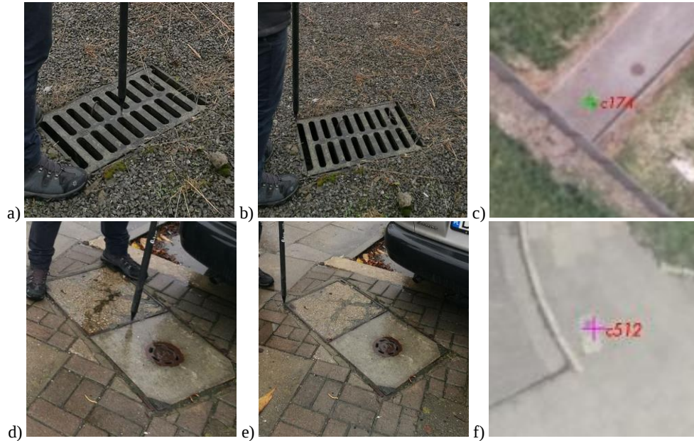
Figure 2. Examples of natural point-type ground control points used in experiment variants: centre of point-type object (option 1) (a, d), corner of point-type (option 2) (b, e) and the view of these identifiable control point on aerial photo (c, f)
