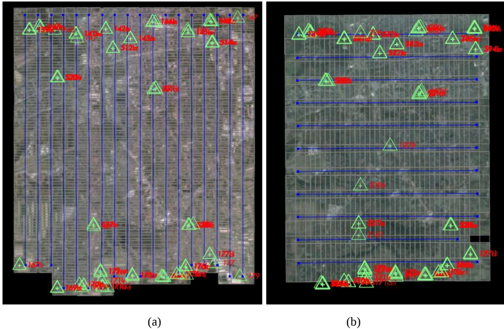
Figure 3. View of photo sub-blocks used in the experiment: block_1 GSD=0.05 m (a), block_2 GSD=0.10 m (b)
